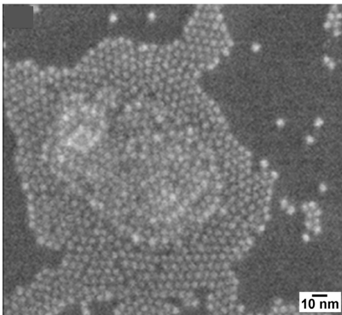
Figure 4.2.1 Quantum dots.
