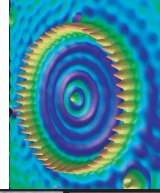
Quantum corral of 48 iron atoms on copper surface positioned one at a time with an STM tip Corral diameter 14 nm
