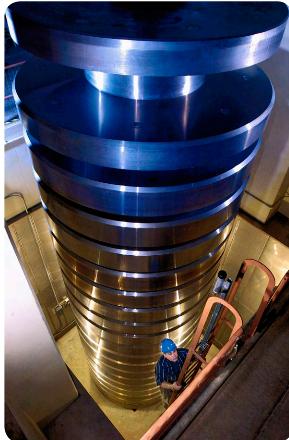
The 4.448 MN (1,000,000 lbf) deadweight machine
