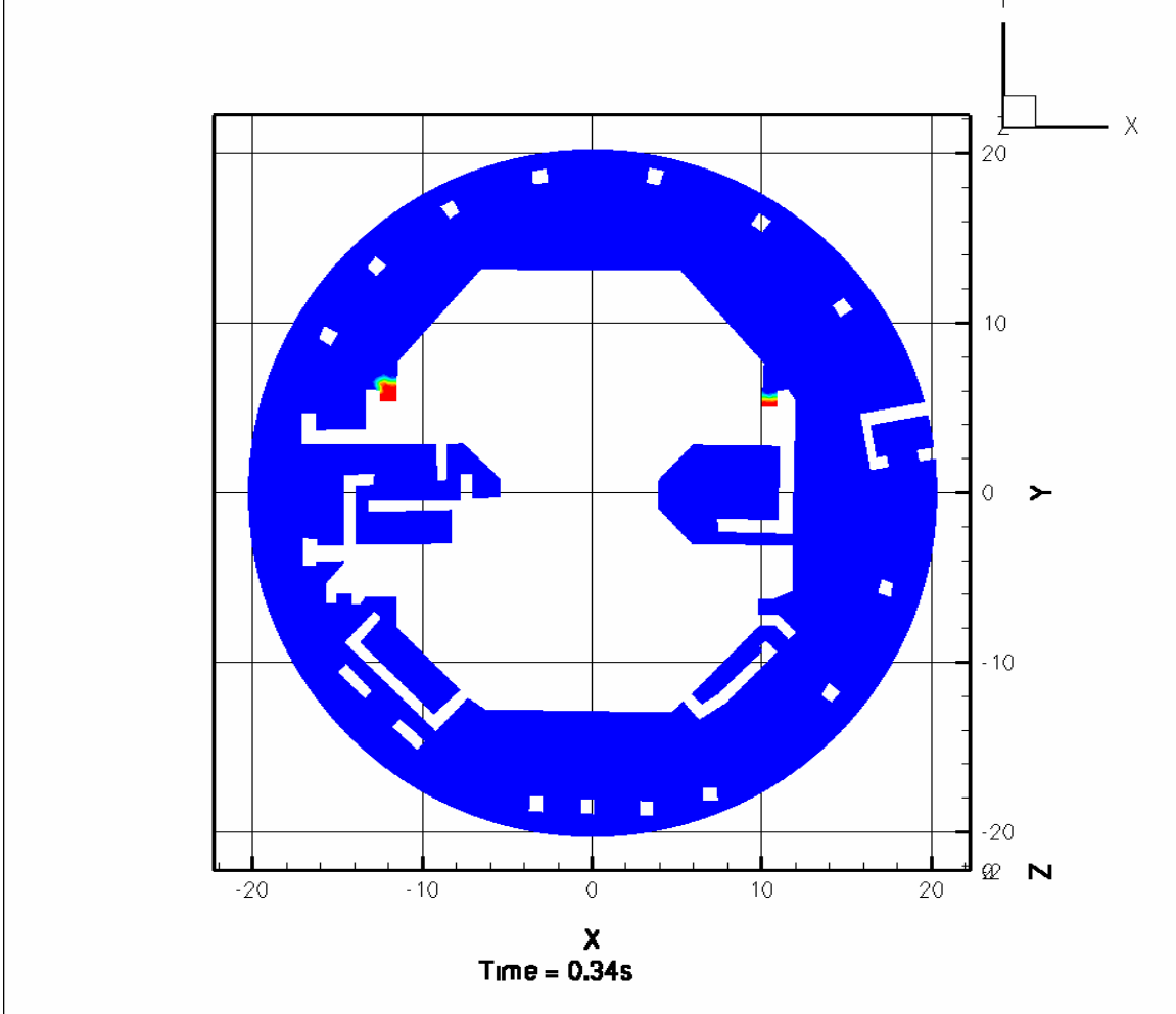
Figure III-4. Transient Volume of Fluid during the Simulation of Containment Pool Fillup
