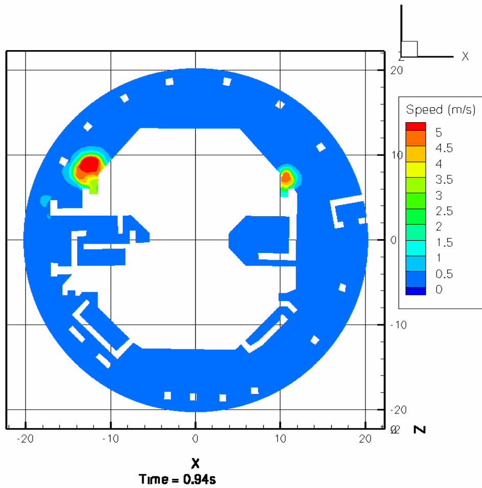
Figure III-14. Same as Figure III-13 for t = 0.94 Seconds
