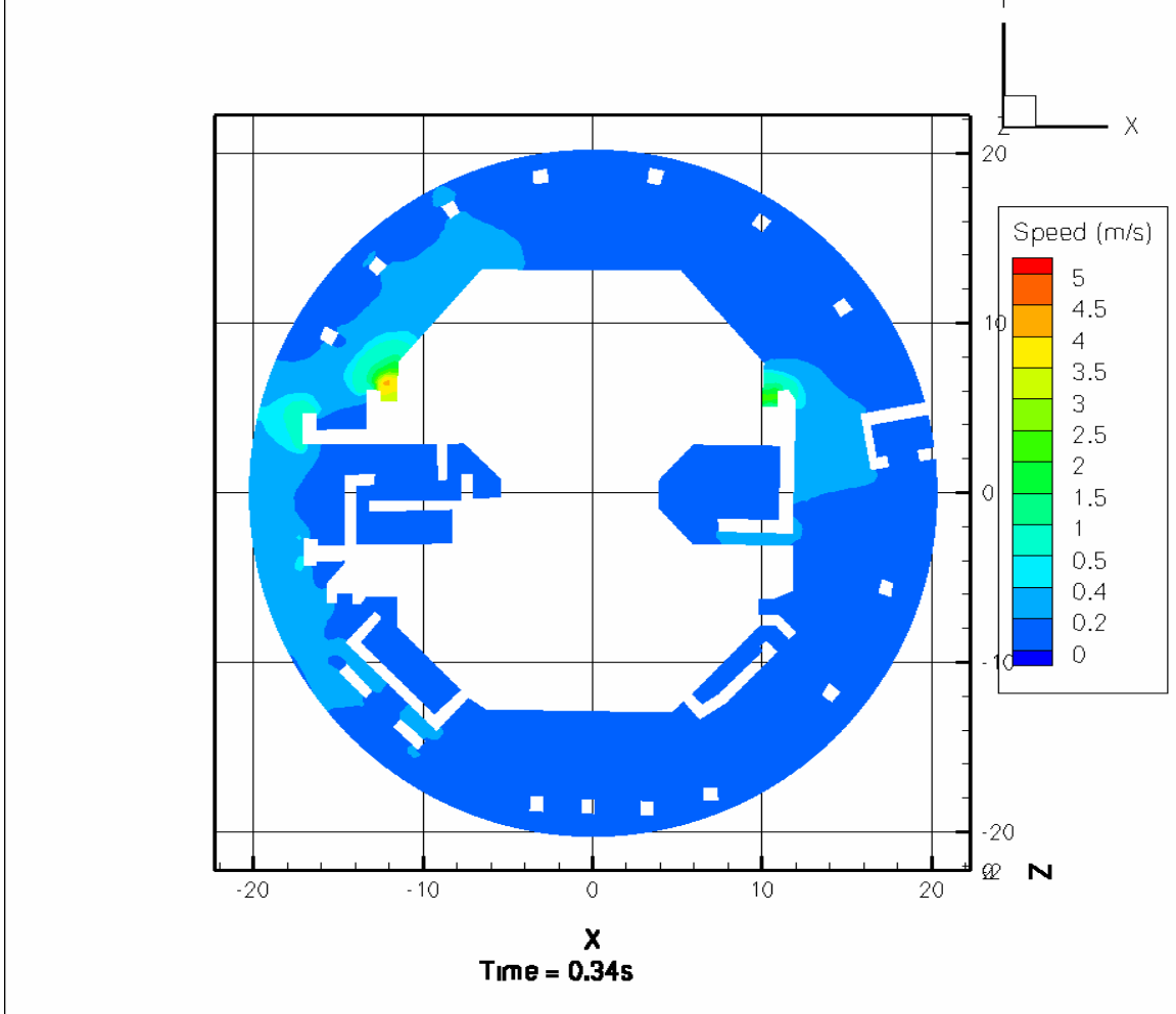
Figure III-13. Transient VOF Simulation of Containment Pool Fillup
