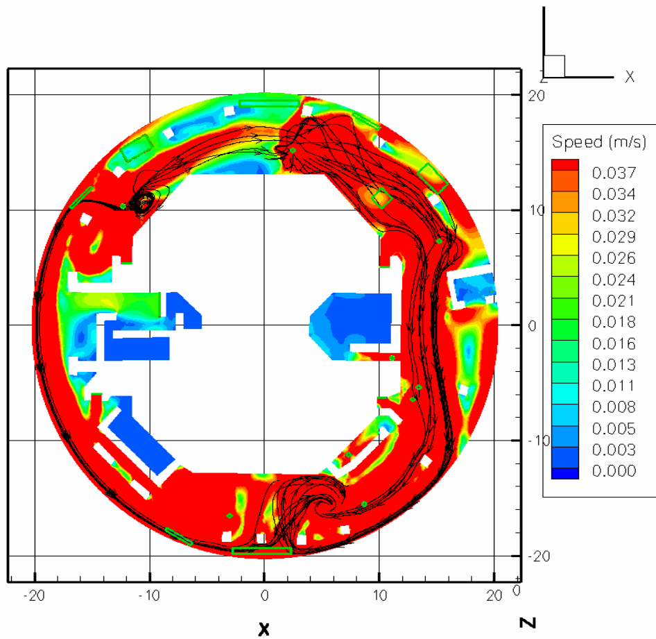
Figure III-38. Streamtraces across Two Splash Locations, Coordinates (-12,10) and (5,15), as Shown in the Figure, for a Large LOCA Break Located in the Upper-Left Quadrant
