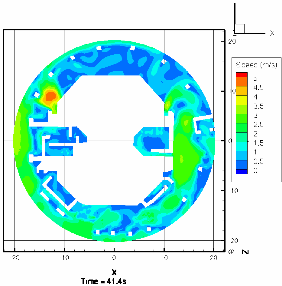
Figure III-18. Same as Figure III-13 for t = 41.4 Seconds
