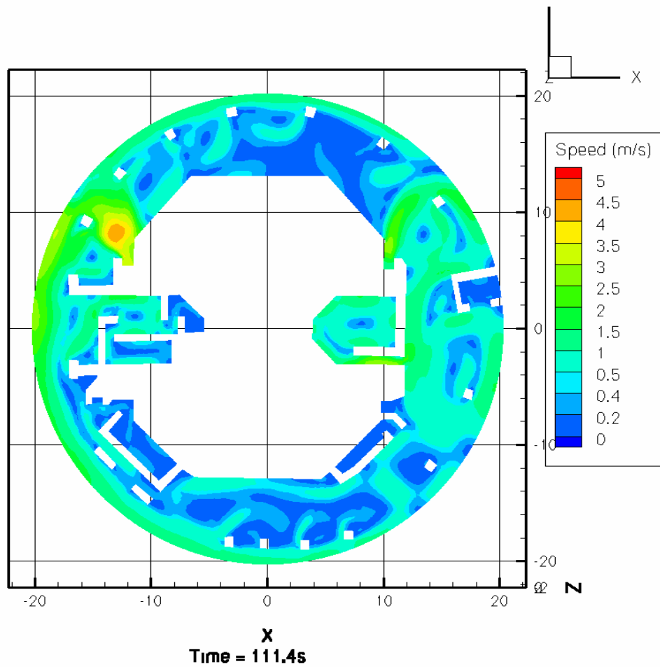
Figure III-21. Same as Figure III-13 for t = 111.4 Seconds
