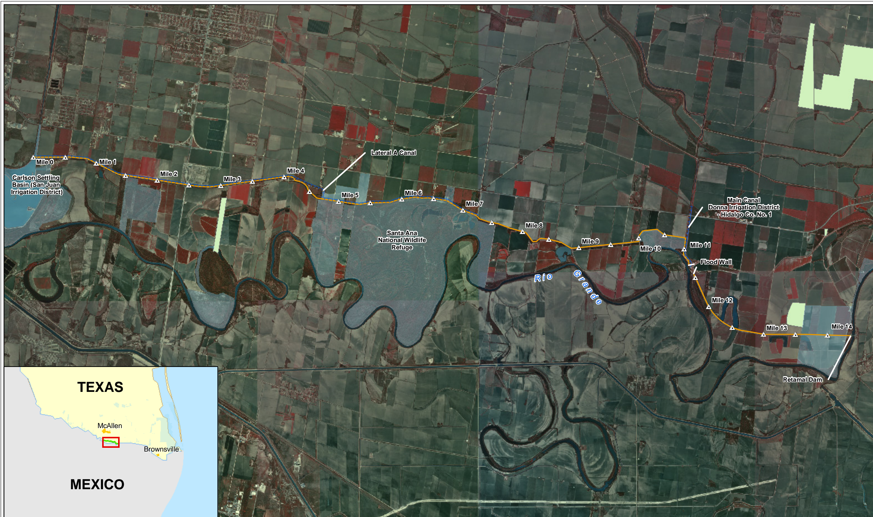
Lateral A/Retamal Dike Levee System Figure 2.1 Project Location Map
