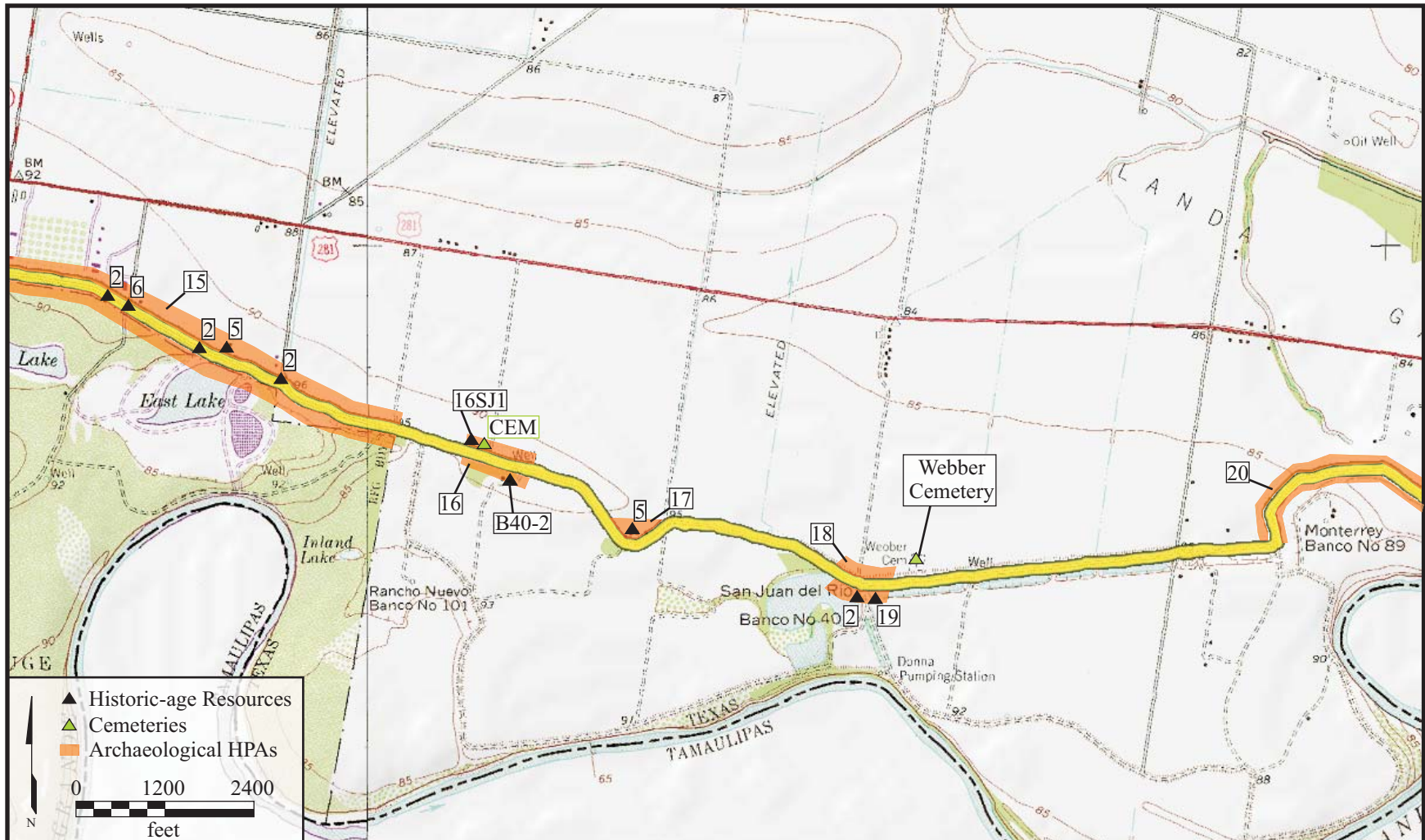
Figure 3.2c. The Lateral A Levee study corridor showing locations of known and potential cultural resources.
