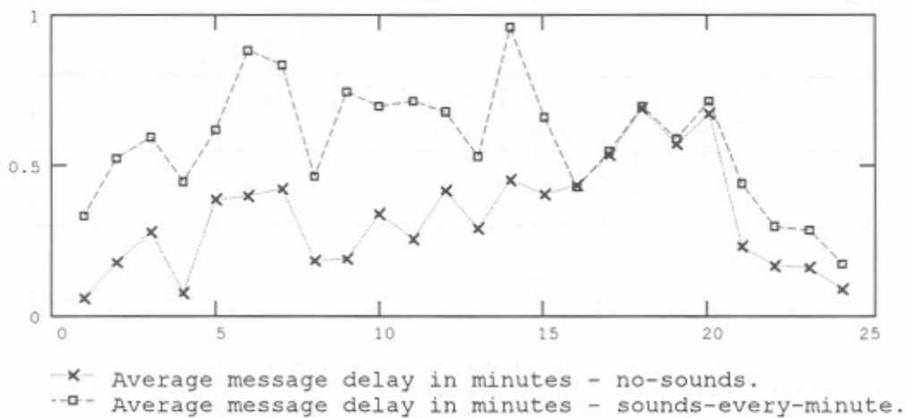
Figure B-11. Simulated network performance by hour-data traces - 5 messages per hour - propagation condition 1 - sounds every minute.
