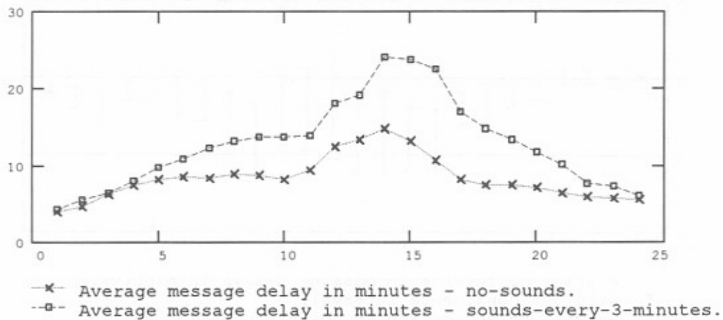
Figure B-65. Simulated network performance by hour-data traces - 60 messages per hour - propagation condition 1 - sounds every 3 minutes.
