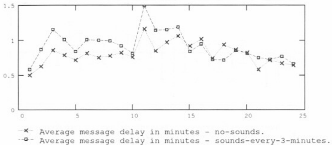
Figure B-31. Simulated network performance by hour-data traces - 15 messages per hour - propagation condition 1 - sounds every 3 minutes.
