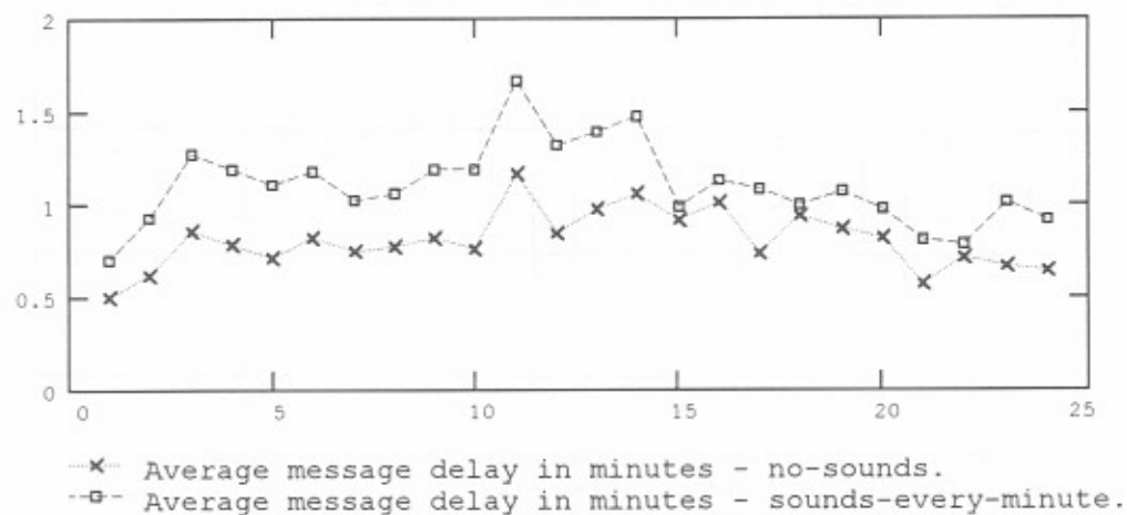
Figure B-35. Simulated network performance by hour-data traces - 15 messages per hour - propagation condition 1 - sounds every minute.
