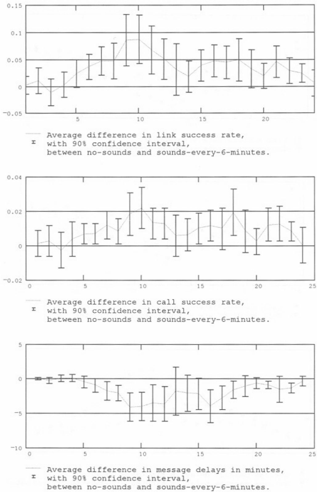
Figure B-64. Simulated network performance by hour-confidence - 60 messages per hour - propagation condition 1 - sounds every 6 minutes.
