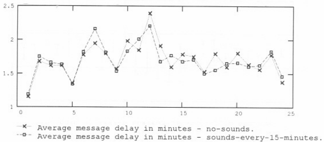
Figure B-37. Simulated network performance by hour-data traces - 30 messages per hour - propagation condition 1 - sounds every 15 minutes.
