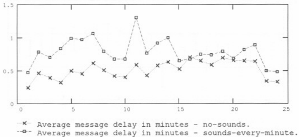
Figure B-23. Simulated network performance by hour-data traces - 10 messages per hour - propagation condition 1 - sounds every minute.
