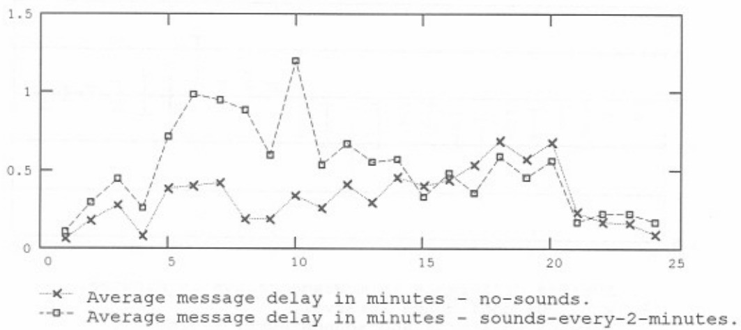
Figure B-9. Simulated network performance by hour-data traces - 5 messages per hour - propagation condition 1 - sounds every 2 minutes.
