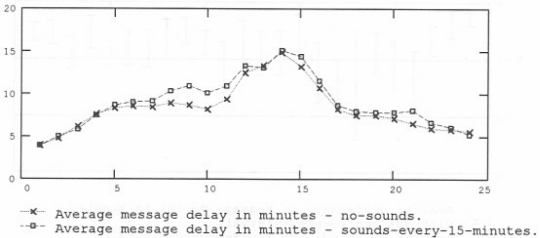
Figure B-61. Simulated network performance by hour-data traces - 60 messages per hour - propagation condition 1 - sounds every 15 minutes.
