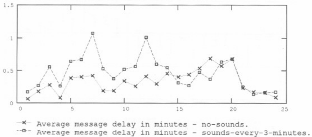
Figure B-7. Simulated network performance by hour-data traces - 5 messages per hour - propagation condition 1 - sounds every 3 minutes.
