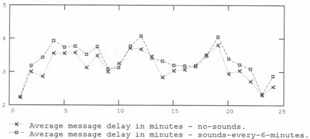
Figure B-53. Simulated network performance by hour-data traces - 45 messages per hour - propagation condition 1 - sounds every 6 minutes.
