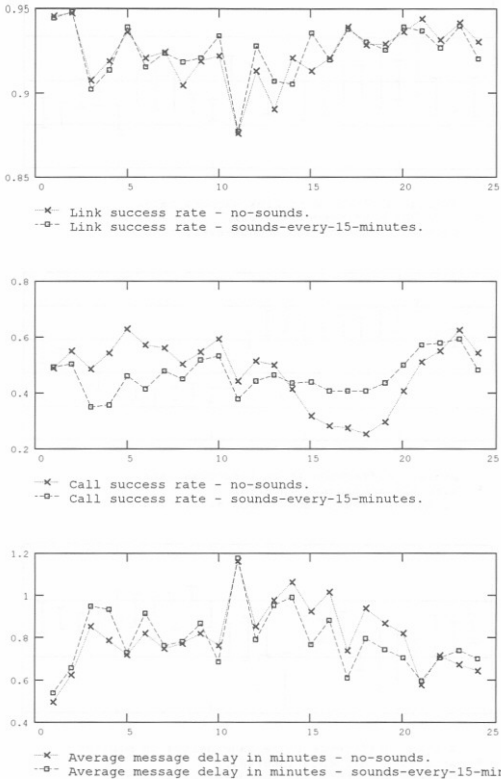
Figure B-25. Simulated network performance by hour-data traces - 15 messages per hour - propagation condition 1 - sounds every 15 minutes.
