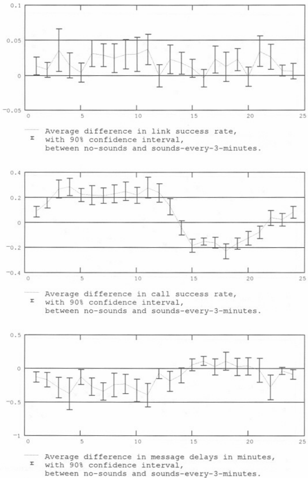
Figure B-20. Simulated network performance by hour-confidence - 10 messages per hour - propagation condition 1 - sounds every 3 minutes.
