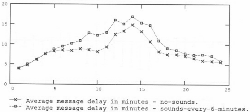
Figure B-63. Simulated network performance by hour-data traces - 60 messages per hour - propagation condition 1 - sounds every 6 minutes.
