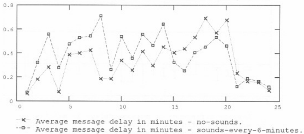
Figure B-5. Simulated network performance by hour-data traces - 5 messages per hour - propagation condition 1 - sounds every 6 minutes.
