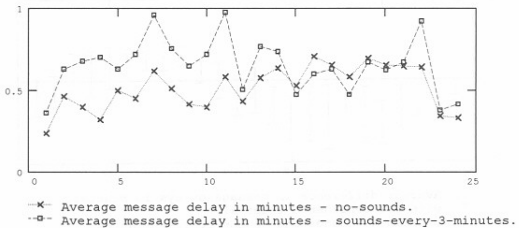
Figure B-19. Simulated network performance by hour-data traces - 10 messages per hour - propagation condition 1 - sounds every 3 minutes.
