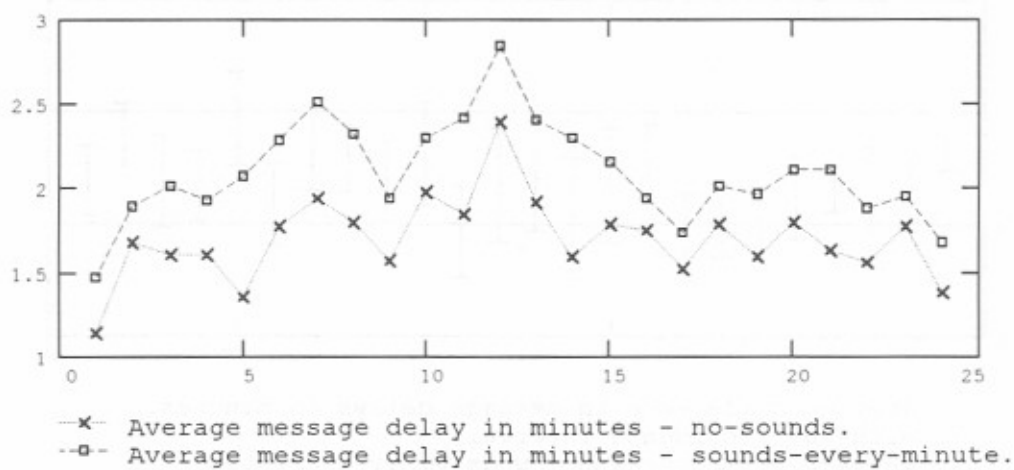
Figure B-47. Simulated network performance by hour-data traces - 30 messages per hour - propagation condition 1 - sounds every minute.
