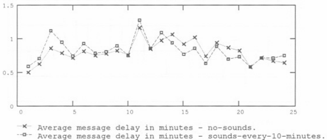
Figure B-27. Simulated network performance by hour-data traces - 15 messages per hour - propagation condition 1 - sounds every 10 minutes.
