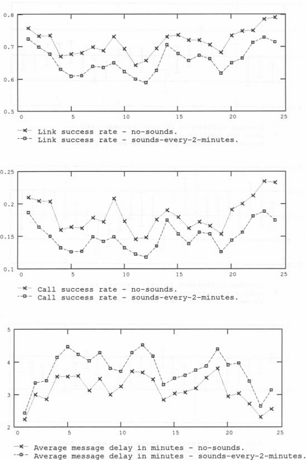
Figure B-57. Simulated network performance by hour-data traces - 45 messages per hour - propagation condition 1 - sounds every 2 minutes.
