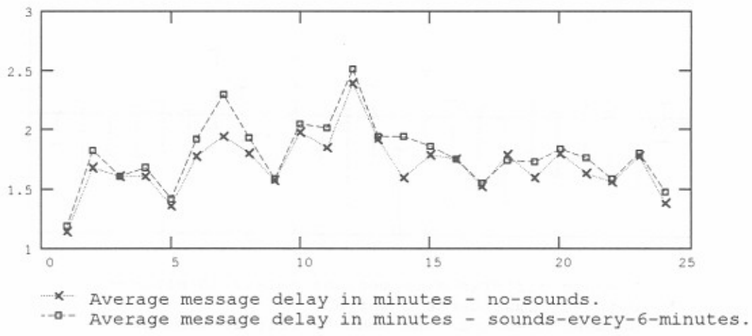
Figure B-41. Simulated network performance by hour-data traces - 30 messages per hour - propagation condition 1 - sounds every 6 minutes.
