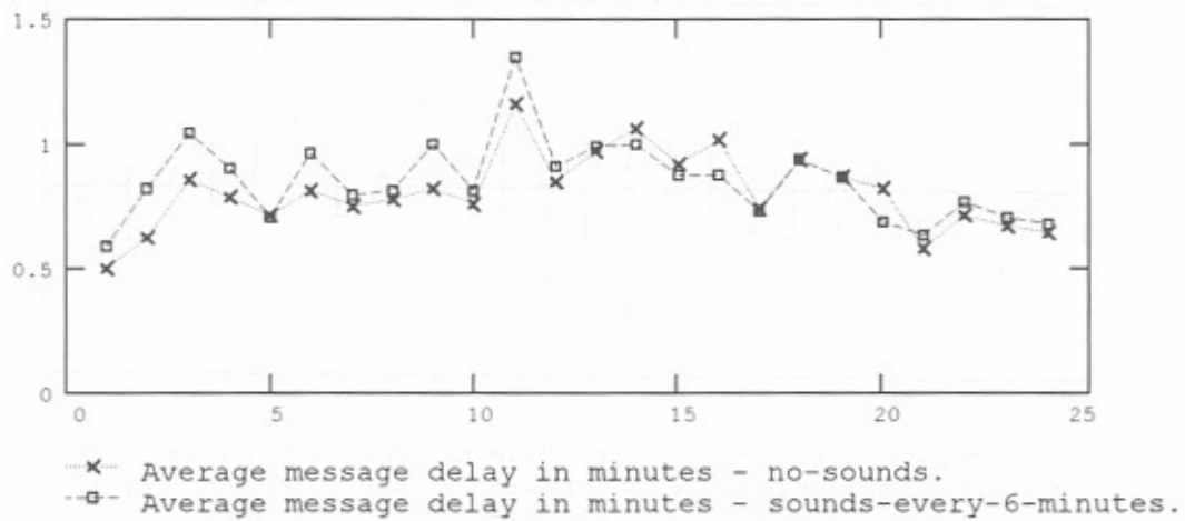
Figure B-29. Simulated network performance by hour-data traces - 15 messages per hour - propagation condition 1 - sounds every 6 minutes.
