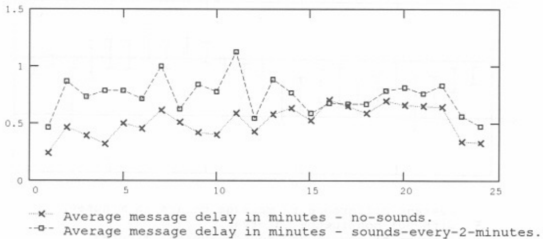
Figure B-21. Simulated network performance by hour-data traces - 10 messages per hour - propagation condition 1 - sounds every 2 minutes.
