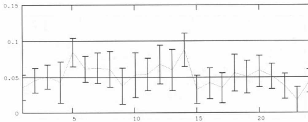
— Average difference in link success rate, ± with 90% confidence interval, between no-sounds and sounds-every-minute.
