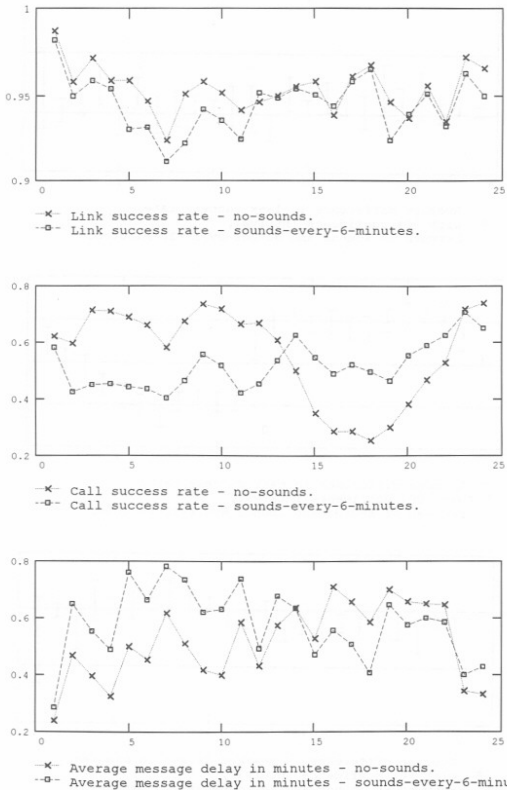
Figure B-17. Simulated network performance by hour-data traces - 10 messages per hour - propagation condition 1 - sounds every 6 minutes.
