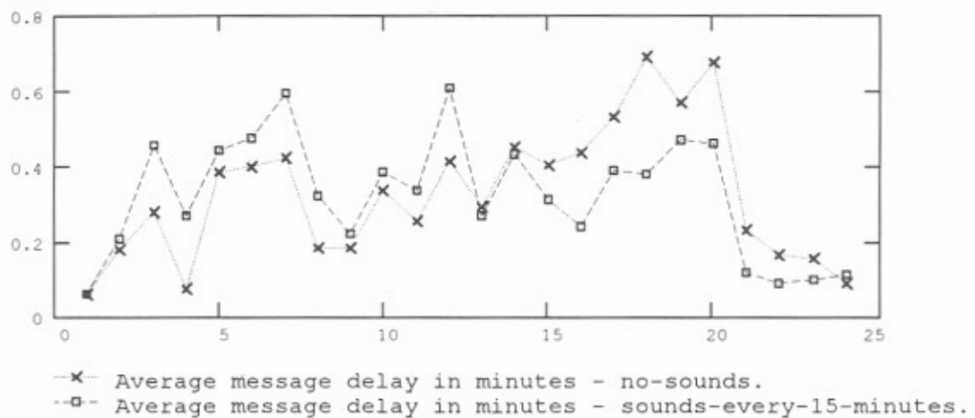
Figure B-1. Simulated network performance by hour-data traces - 5 messages per hour - propagation condition 1 - sounds every 15 minutes.
