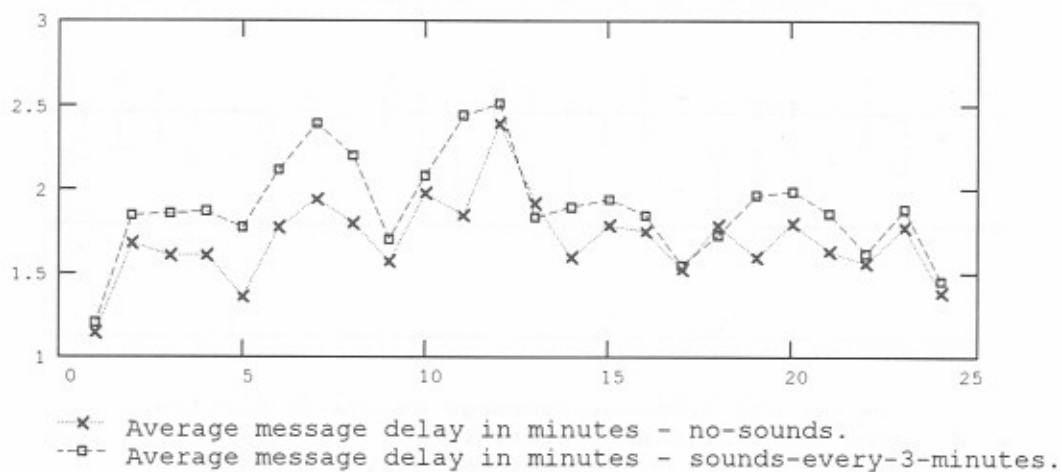
Figure B-43. Simulated network performance by hour-data traces - 30 messages per hour - propagation condition 1 - sounds every 3 minutes.
