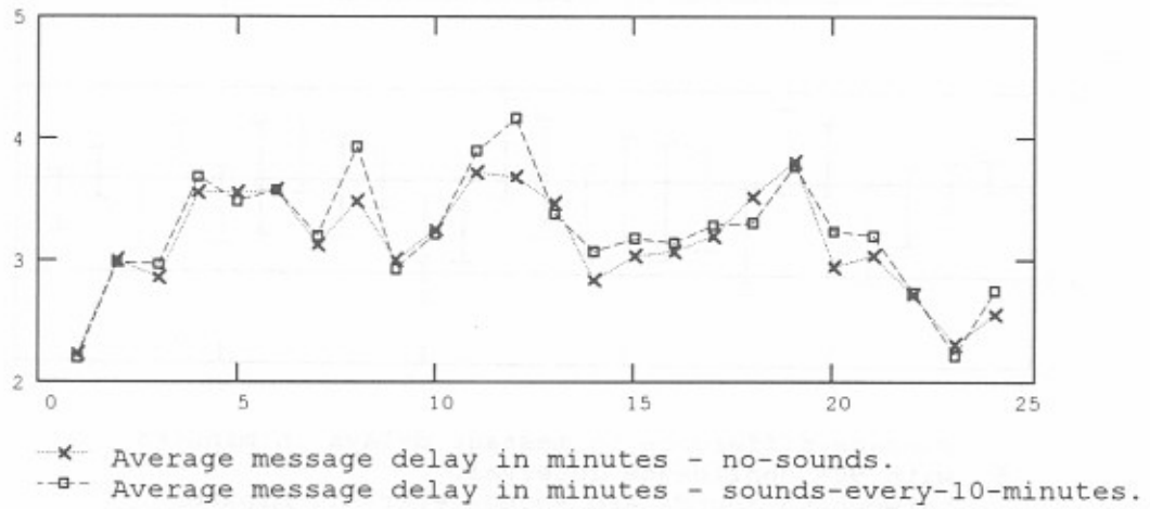
Figure B-51. Simulated network performance by hour-data traces - 45 messages per hour - propagation condition 1 - sounds every 10 minutes.
