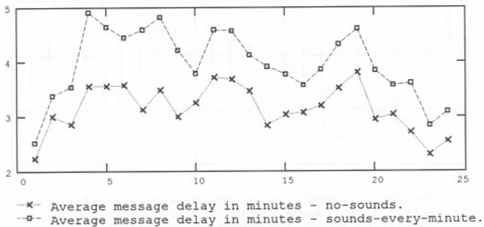
Figure B-59. Simulated network performance by hour-data traces - 45 messages per hour - propagation condition 1 - sounds every minute.
