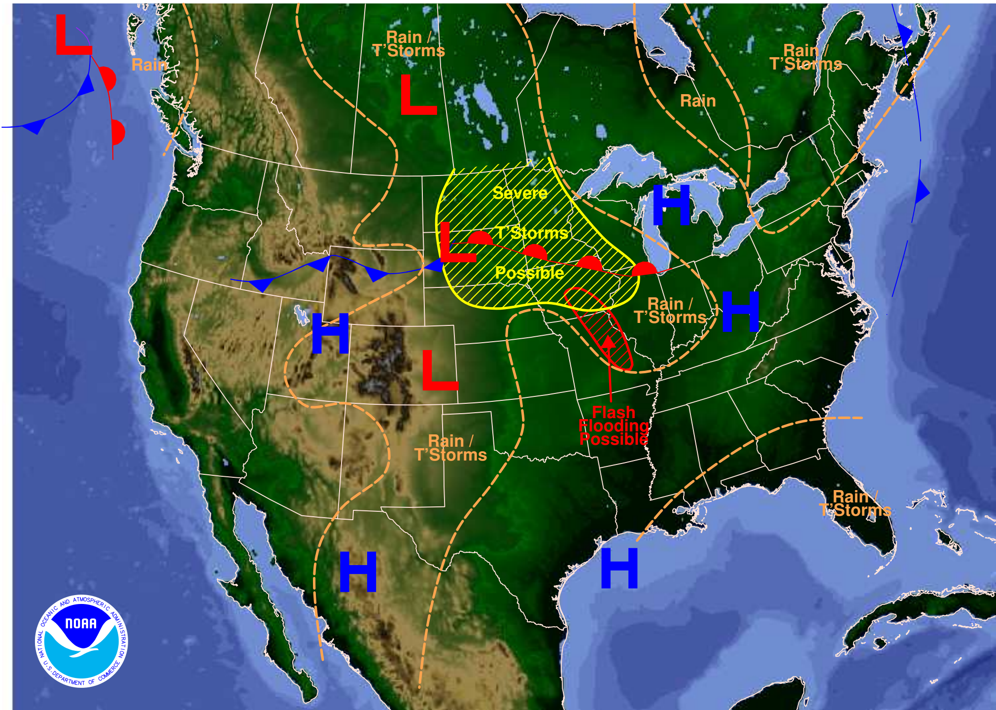
Weather Forecast for Monday, July 28, 2008 DOC/NOAA/NWS/NCEP/Hydrometeorological Prediction Center Prepared by Kong based on HPC, SPC, and TPC forecasts.
