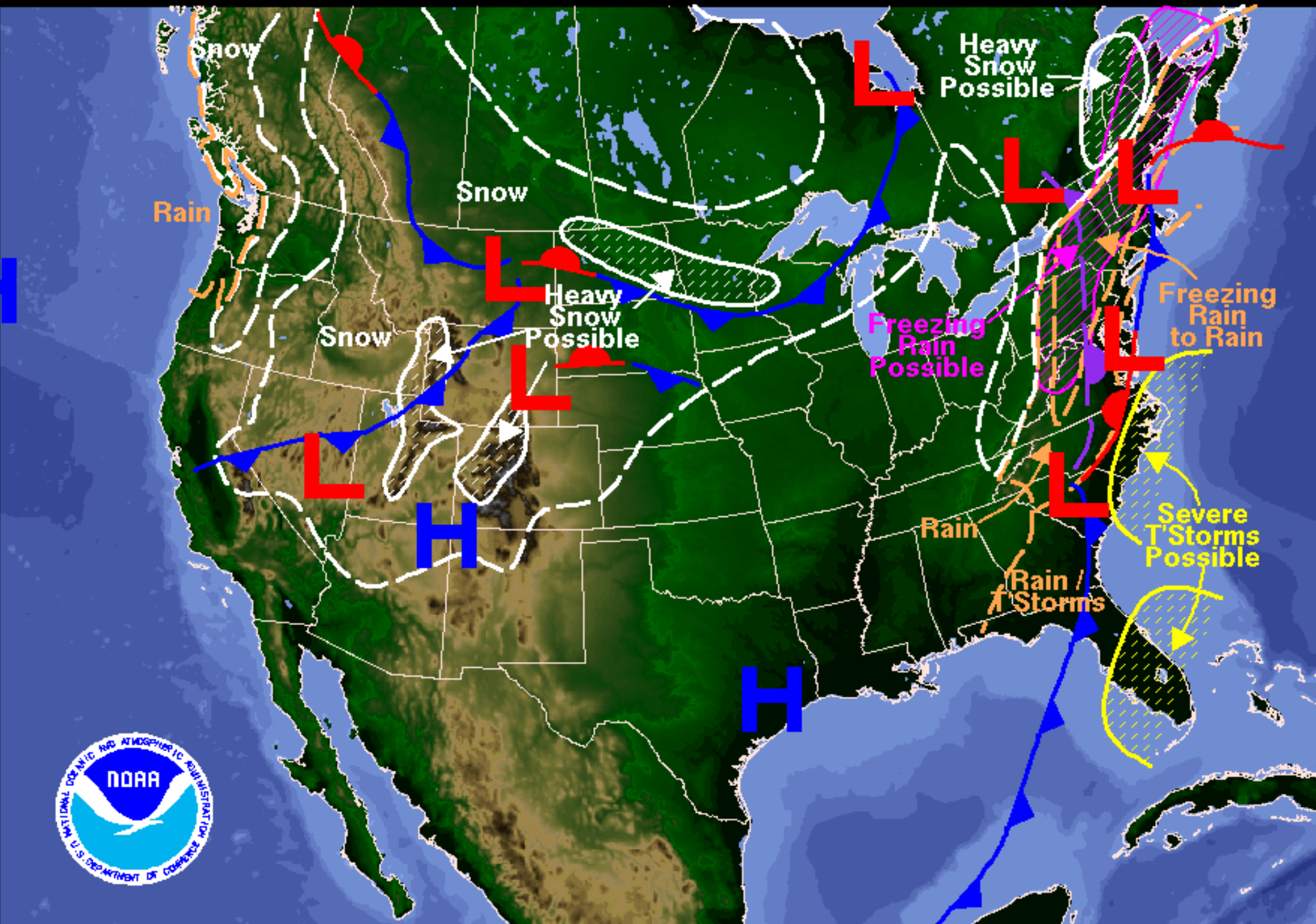
Weather Forecast for Wednesday, February 13, 2008 DOC/NOAA/NWS/NCEP/Hydrometeorological Prediction Center Prepared by Kong based on HPC, SPC, and TPC forecasts.
