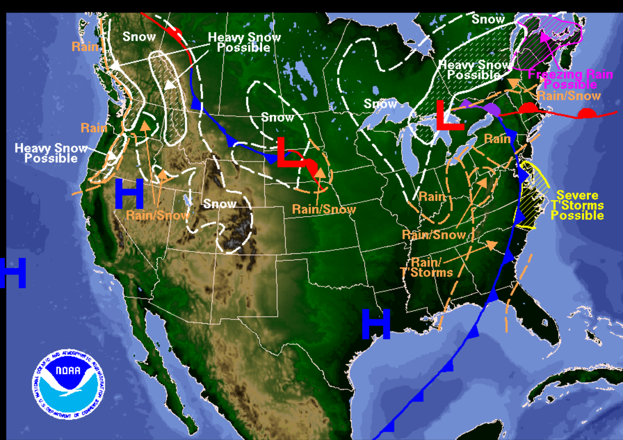
Weather Forecast for Friday, January 11, 2008 DOC/NOAA/NWS/NCEP/Hydrometeorological Prediction Center Prepared by Kocin based on HPC, SPC, and TPC forecasts.
