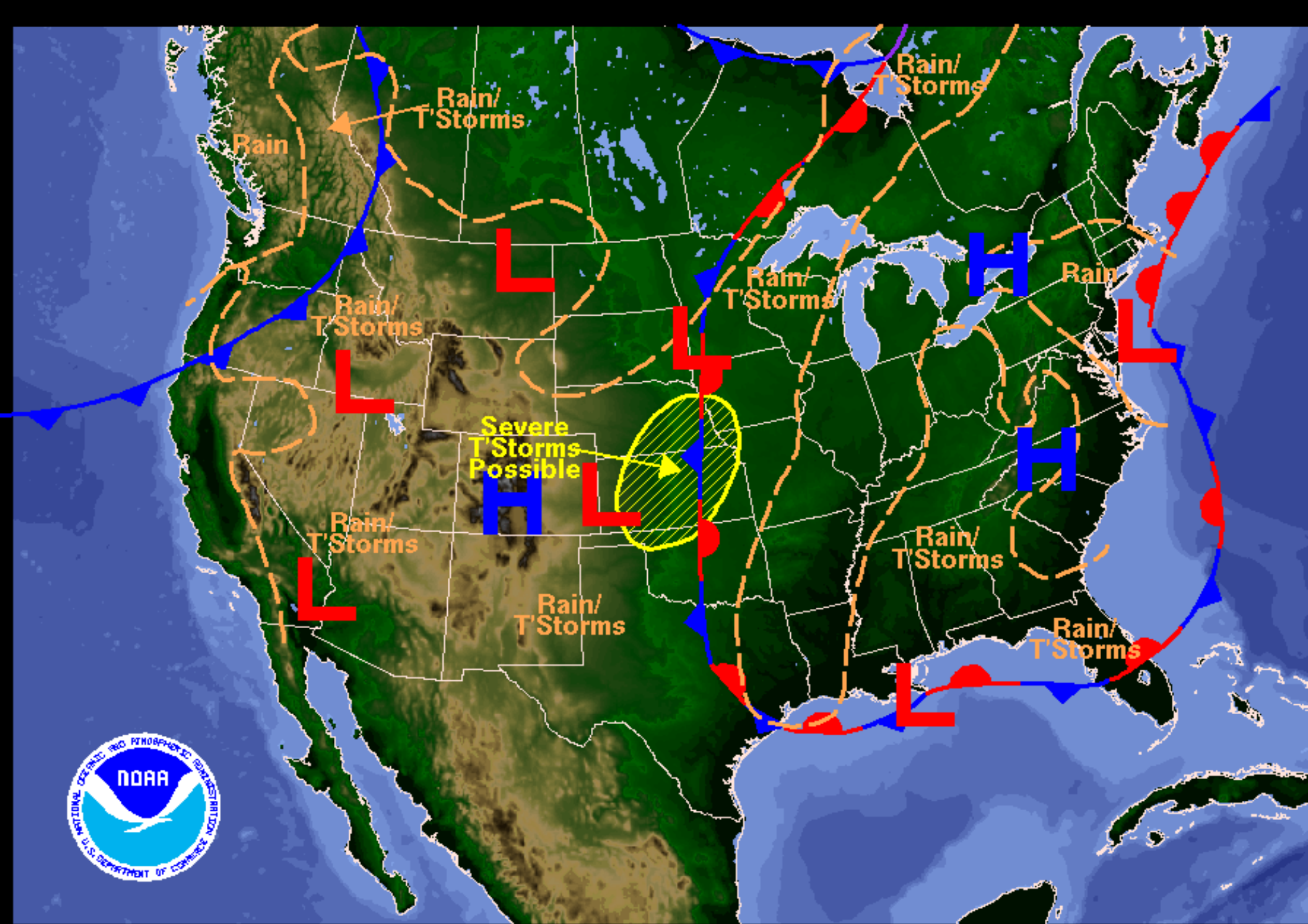
Weather Forecast for Monday, July 23, 2007 DOC/NOAA/NWS/NCEP/Hydrometeorological Prediction Center Prepared by Kocin based on HPC, SPC, and TPC forecasts.
