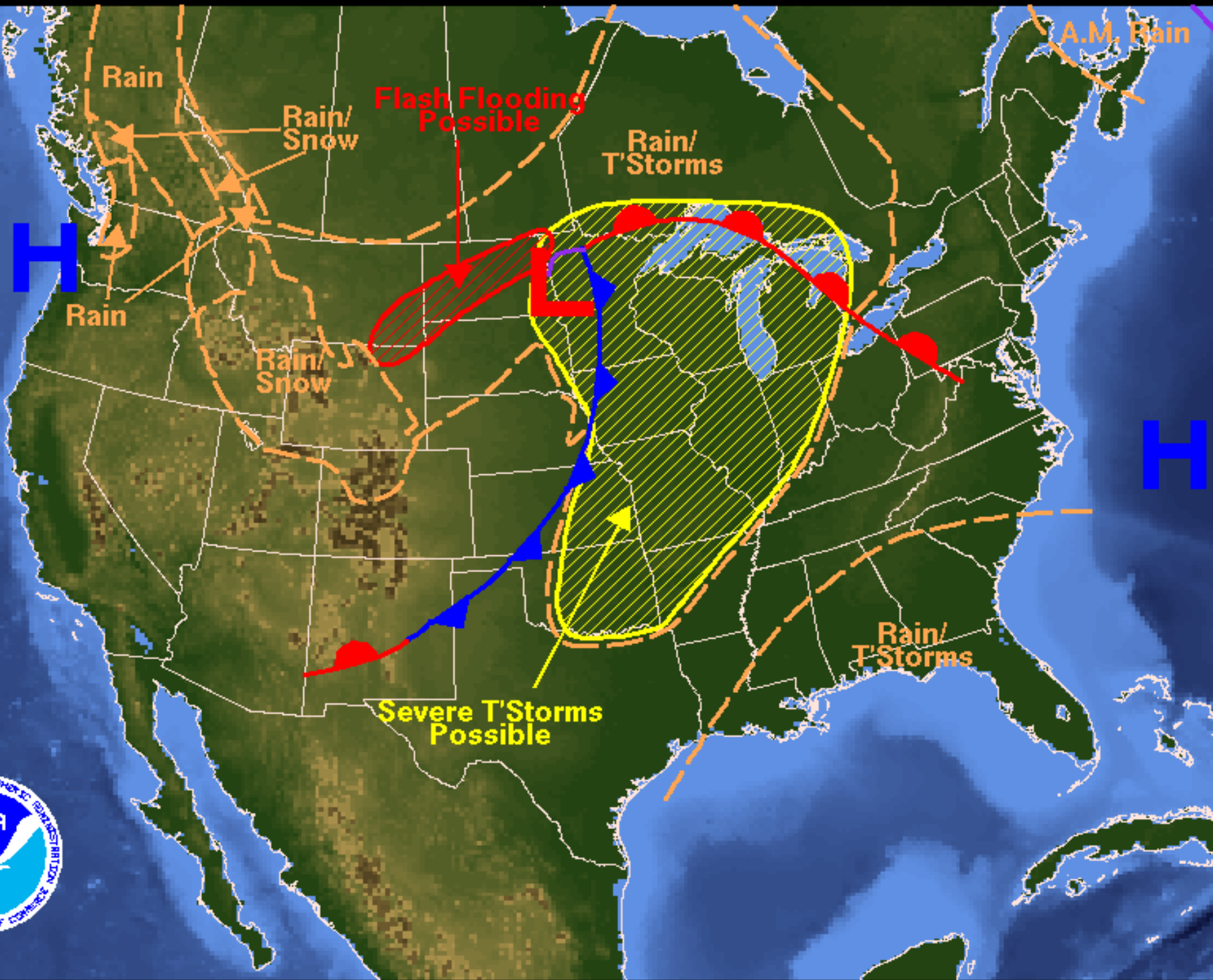
Weather Forecast for Thursday, June 07, 2007 DOC/NOAA/NWS/NCEP/Hydrometeorological Prediction Center Prepared by Rubin-Oster based on HPC, SPC, and TPC forecasts.
