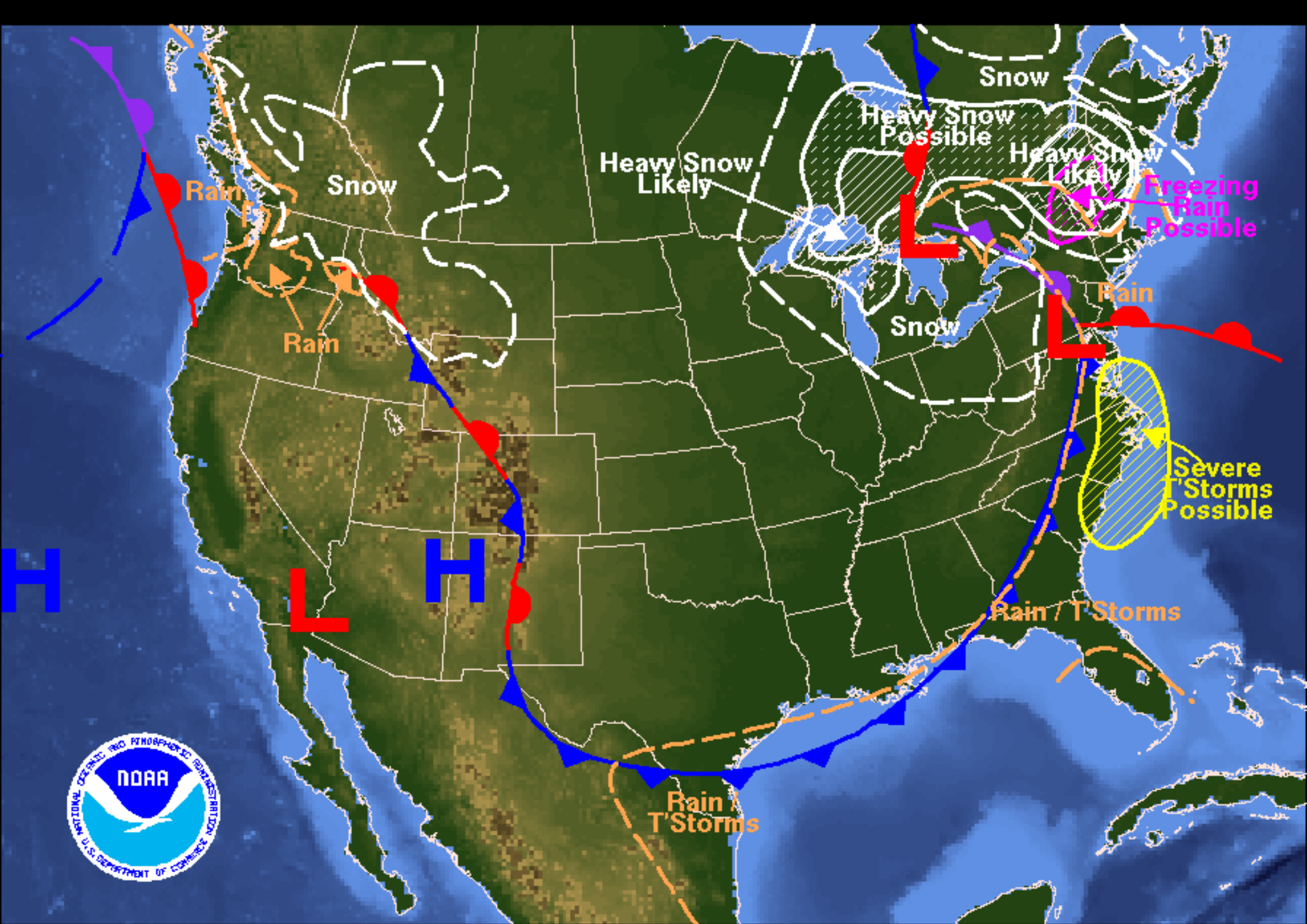
Weather Forecast for Wednesday, April 04, 2007 DOC/NOAA/NWS/NCEP/Hydrometeorological Prediction Center Prepared by Kong based on HPC, SPC, and TPC forecasts.
