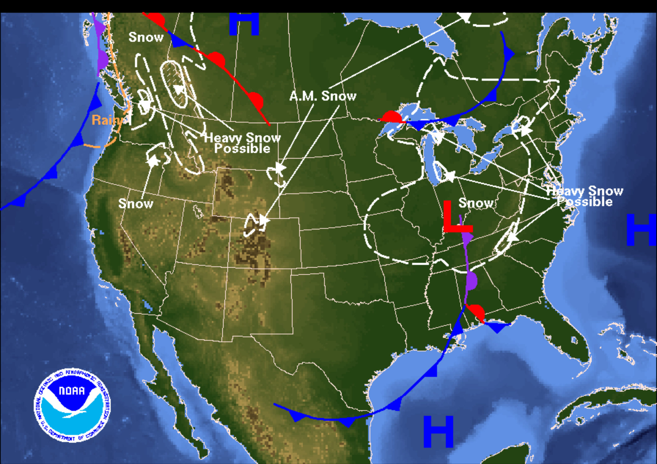
Weather Forecast for Saturday, February 17, 2007 DOC/NOAA/NWS/NCEP/Hydrometeorological Prediction Center Prepared by Rubin-Oster based on HPC, SPC, and TPC forecasts.
