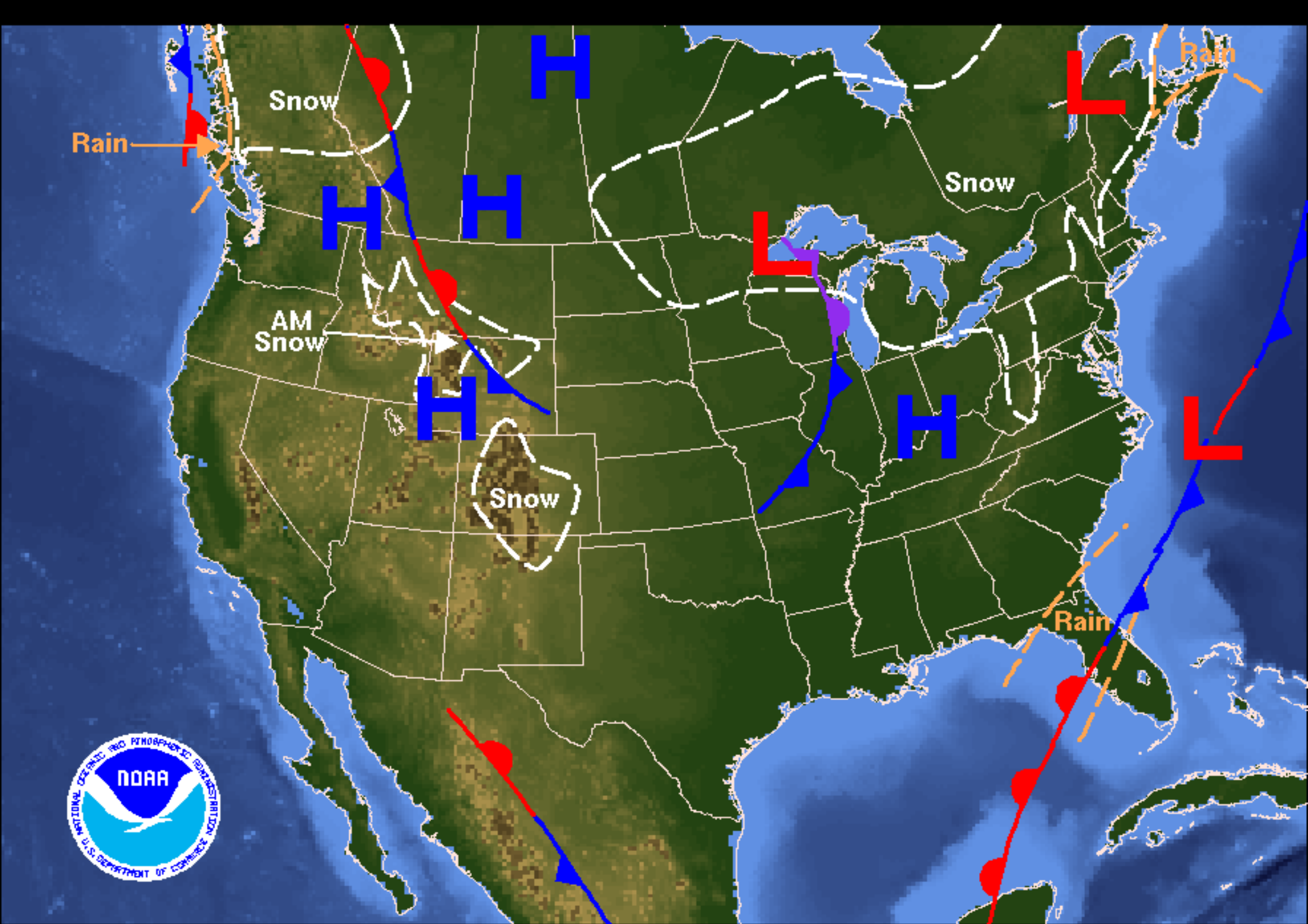
Weather Forecast for Saturday, December 02, 2006 DOC/NOAA/NWS/NCEP/Hydrometeorological Prediction Center Prepared by Fracasso based on HPC, SPC, and TPC forecasts.
