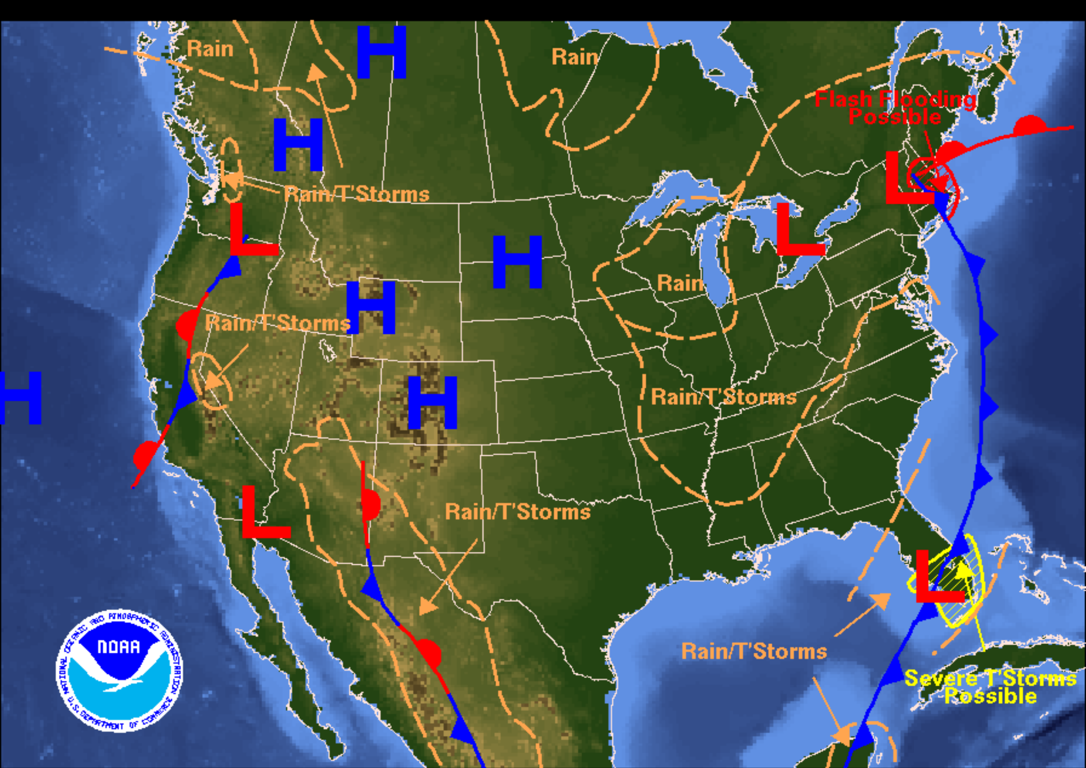
Weather Forecast for Tuesday, May 16, 2006 DOC/NOAA/NWS/NCEP/Hydrometeorological Prediction Center Prepared by Bell based on HPC, SPC, and TPC forecasts.
