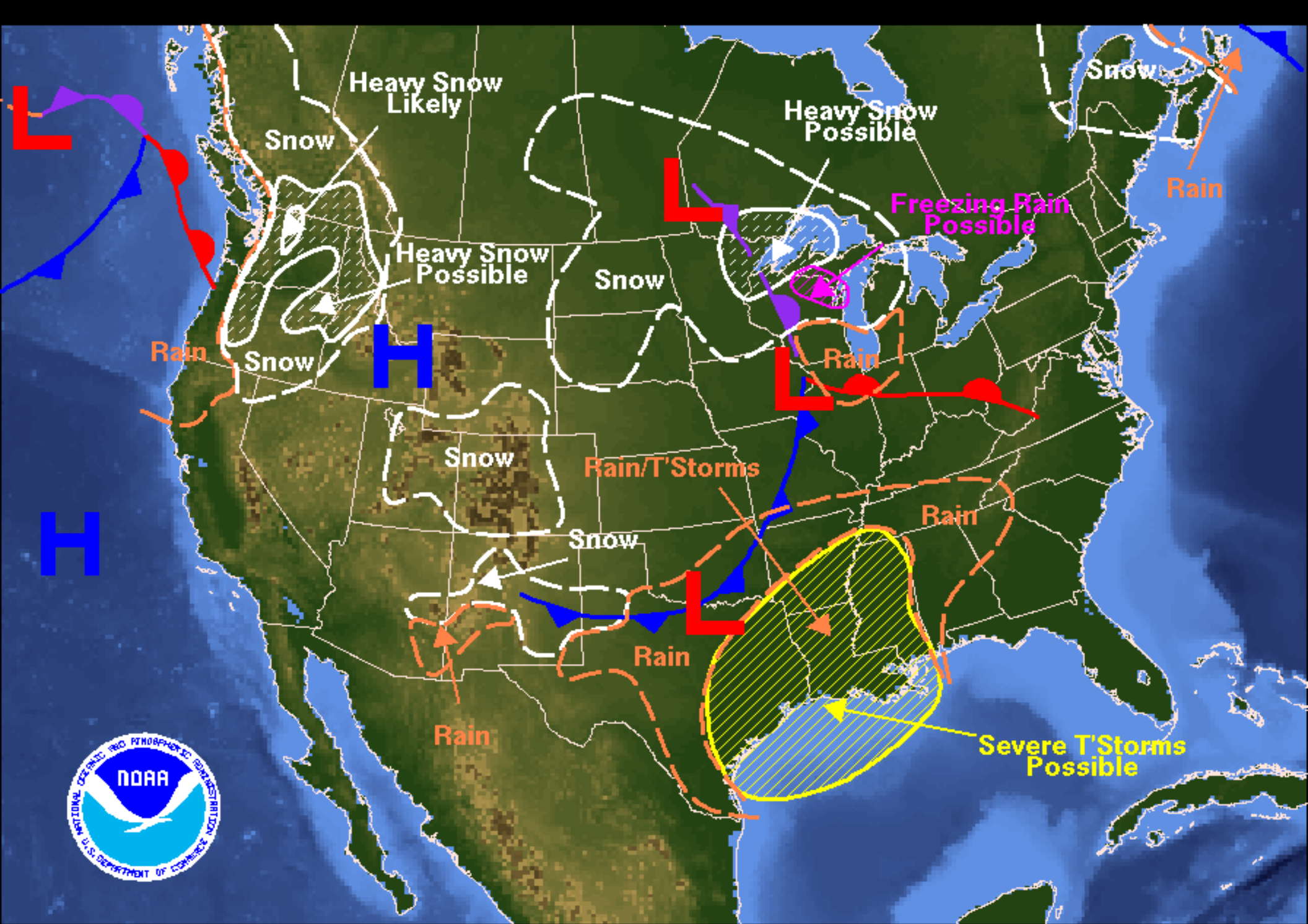
Weather Forecast for Monday, January 16, 2006 DOC/NOAA/NWS/NCEP/Hydrometeorological Prediction Center Prepared by Bell based on HPC, SPC, and TPC forecasts.
