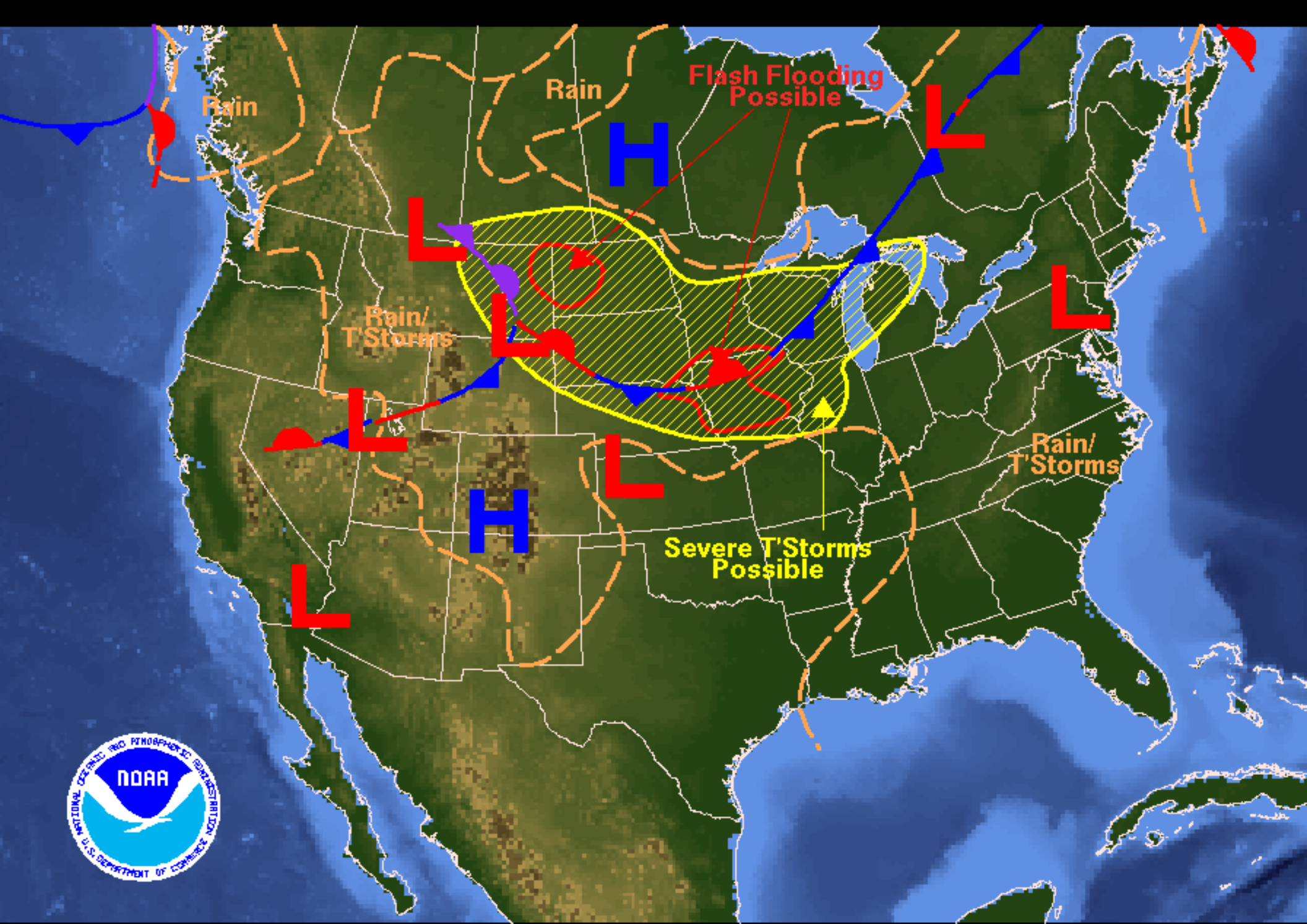
Weather Forecast for Tuesday, June 28, 2005 DOC/NOAA/NWS/NCEP/Hydrometeorological Prediction Center Prepared by Fries/Sullivan based on HPC, SPC, and TPC forecasts.
