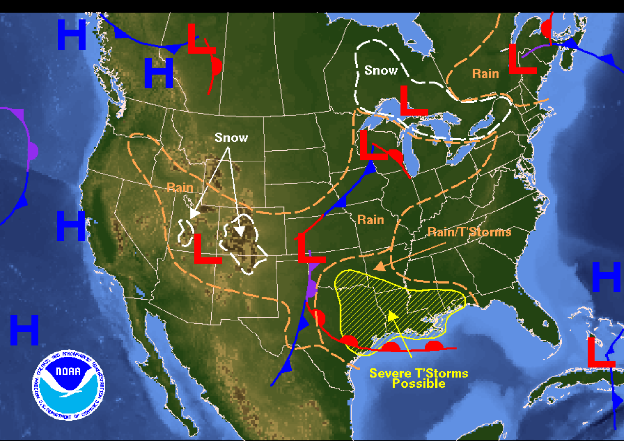
Weather Forecast for Monday, April 25, 2005 DOC/NOAA/NWS/NCEP/Hydrometeorological Prediction Center Prepared by Szatanek/Oravec based on HPC, SPC, and TPC forecasts.
