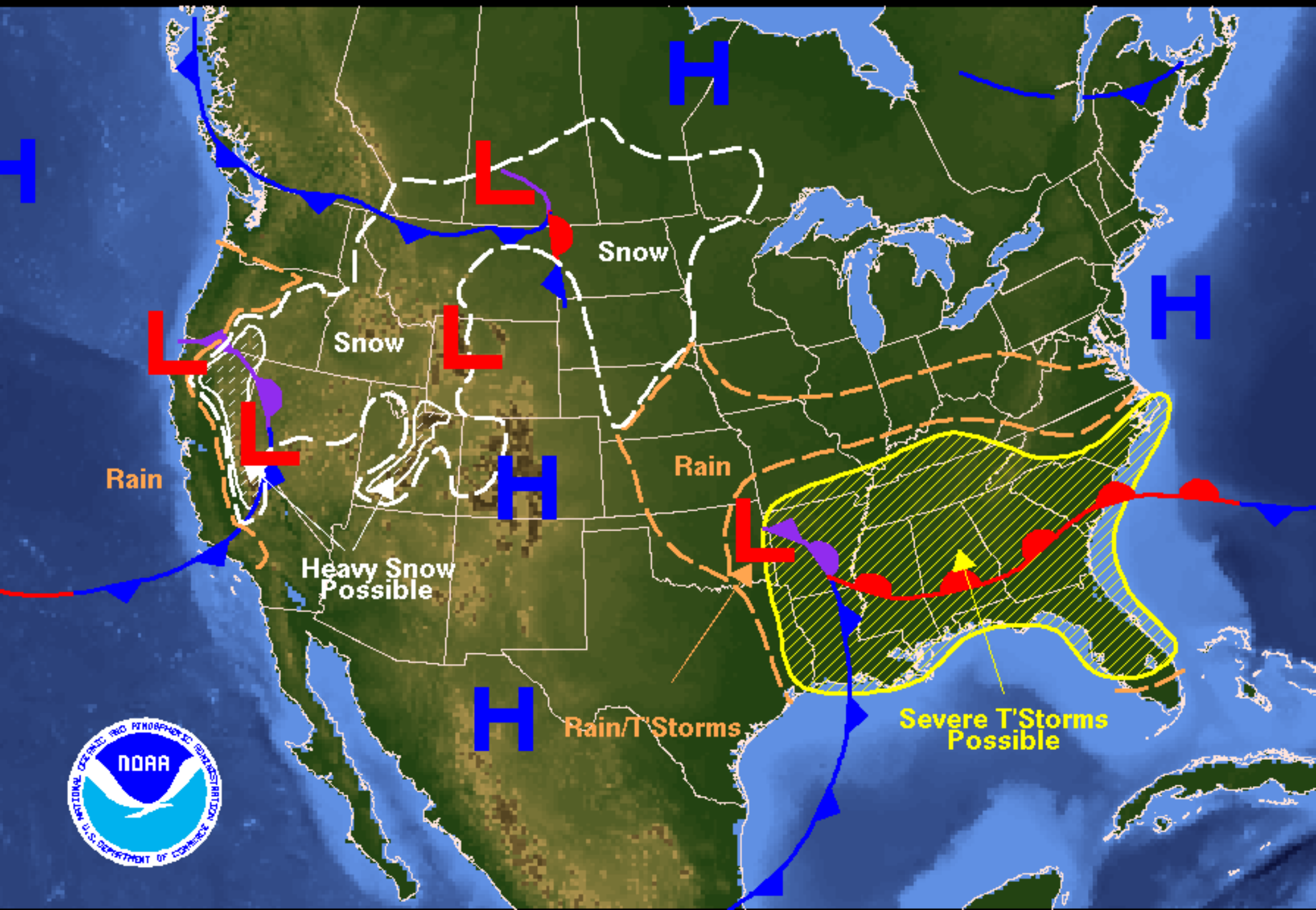
Weather Forecast for Tuesday, March 22, 2005 DOC/NOAA/NWS/NCEP/Hydrometeorological Prediction Center Prepared by Szatanek/Oravec based on HPC, SPC, and TPC forecasts.
