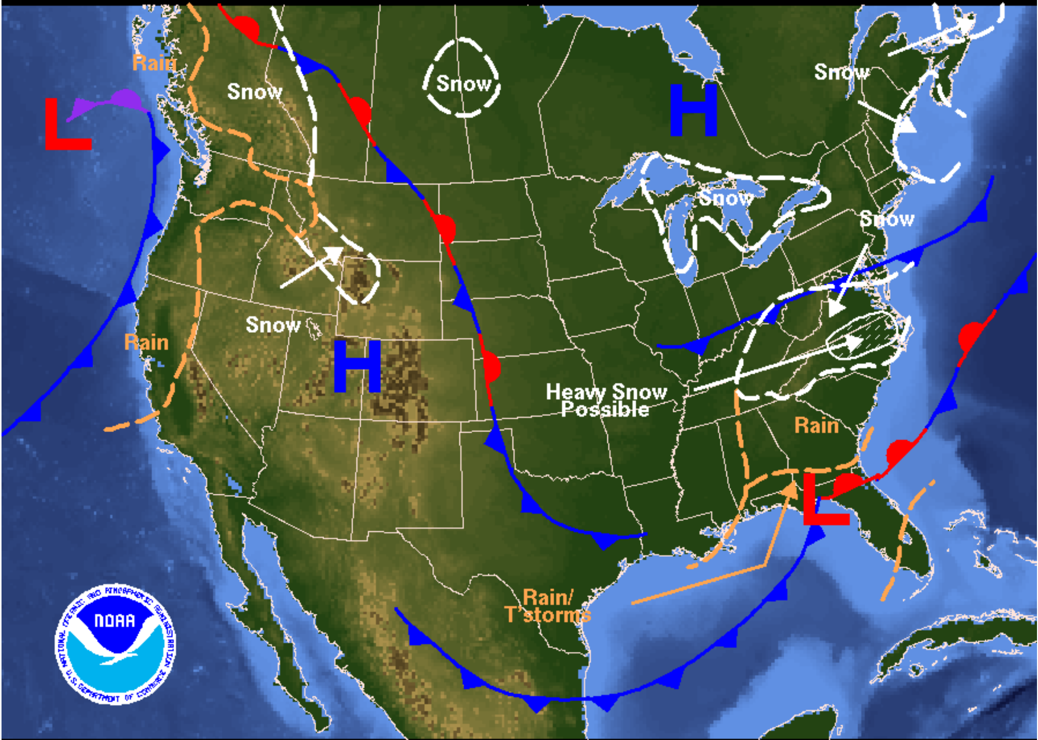
Weather Forecast for Friday, January 09, 2004 DOC/NOAA/NWS/NCEP/Hydrometeorological Prediction Center Prepared by JACKSON/KORTY based on HPC, SPC, and TPC forecasts.
