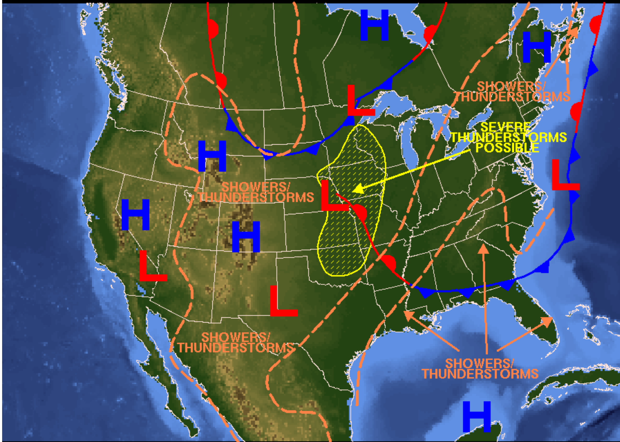
Weather Forecast for Wednesday, August 15, 2001 Prepared by JACKSON/TERRY DOC/NOAA/NWS/NCEP/Hydrometeorological Prediction Center
