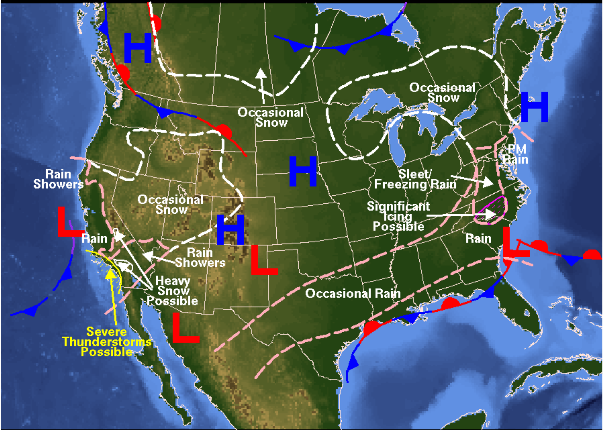
Weather Forecast for Monday, February 12, 2001 Prepared by RAUSCH/ECKERT DOC/NOAA/NWS/NCEP/Hydrometeorological Prediction Center
