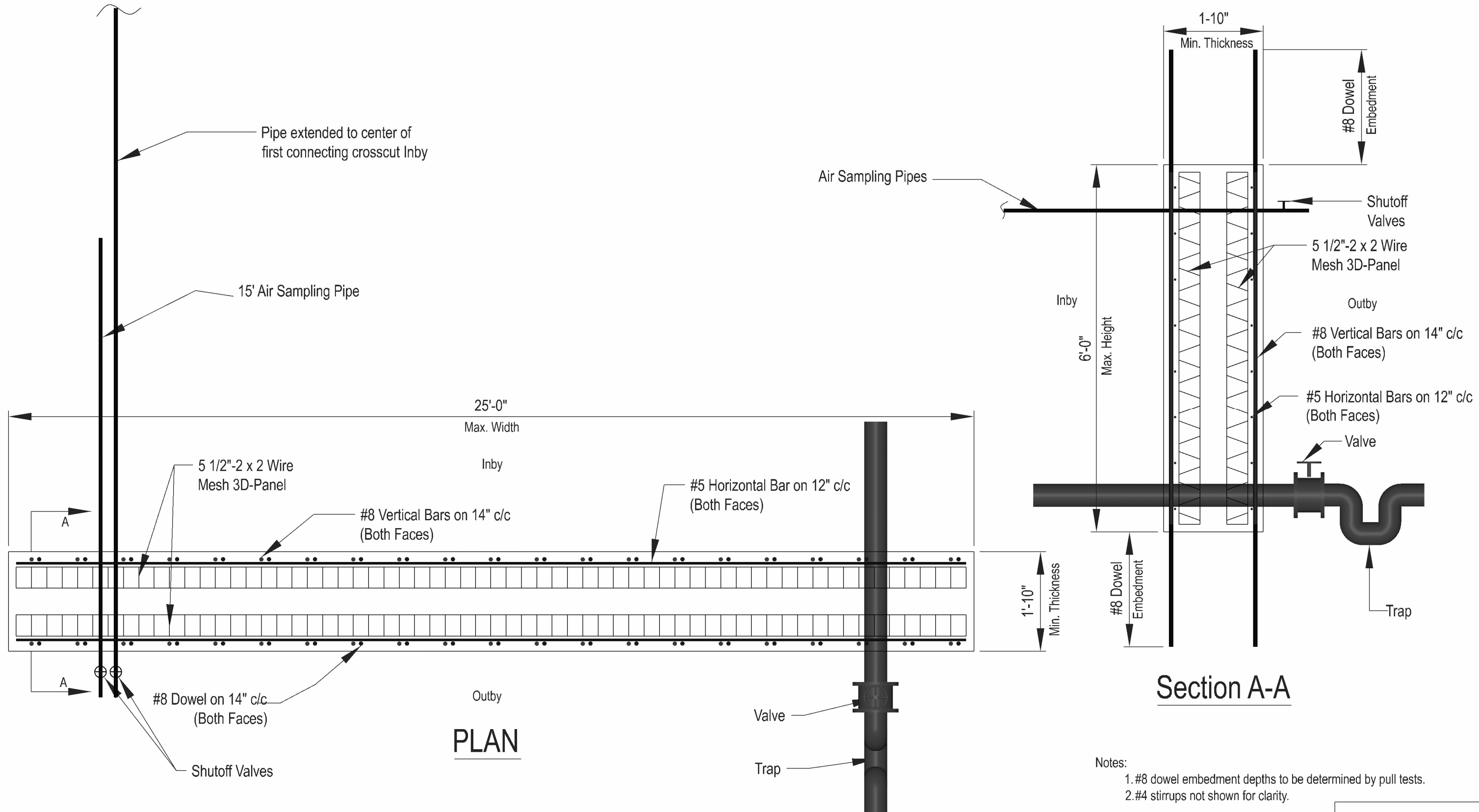
Precision Mine Repair 120 PSI Plan & Section View Figure #2
