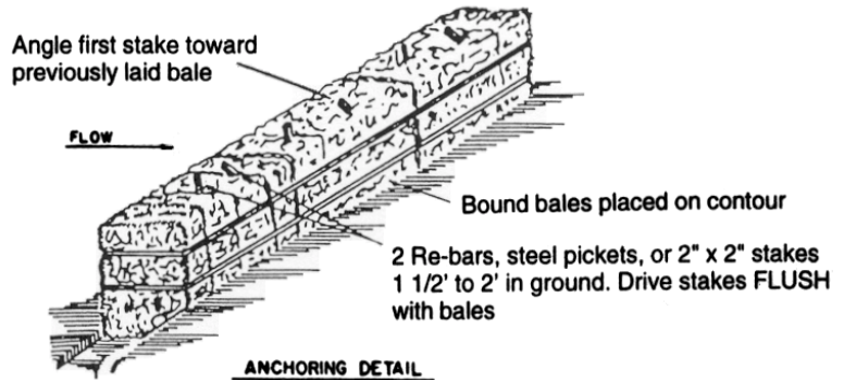
ANCHORING DETAIL
