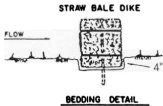
BEDDING DETAIL
