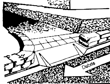
Controlling debris/storm flows in streets
