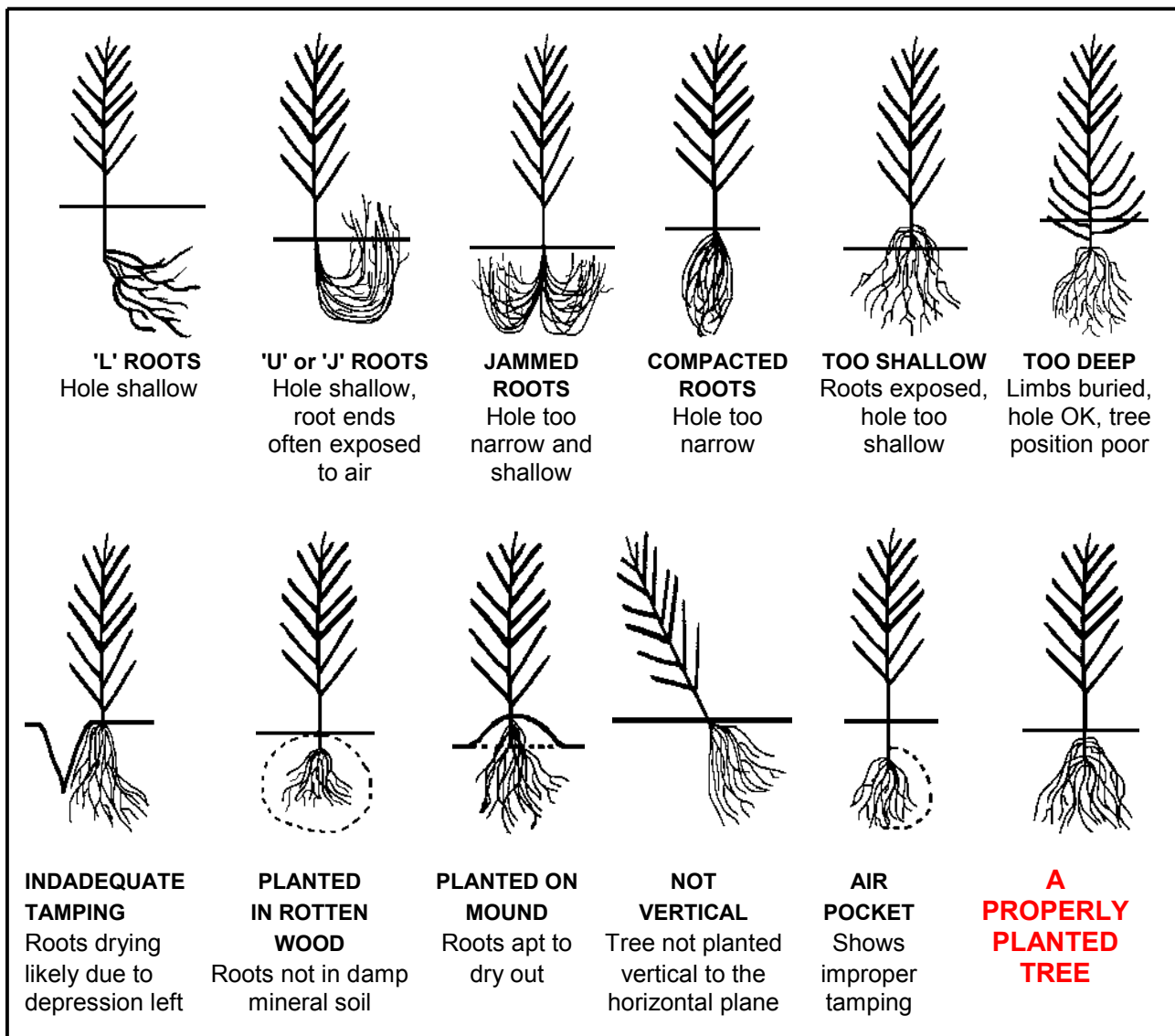
Figure 5: Examples of improperly planted trees.
