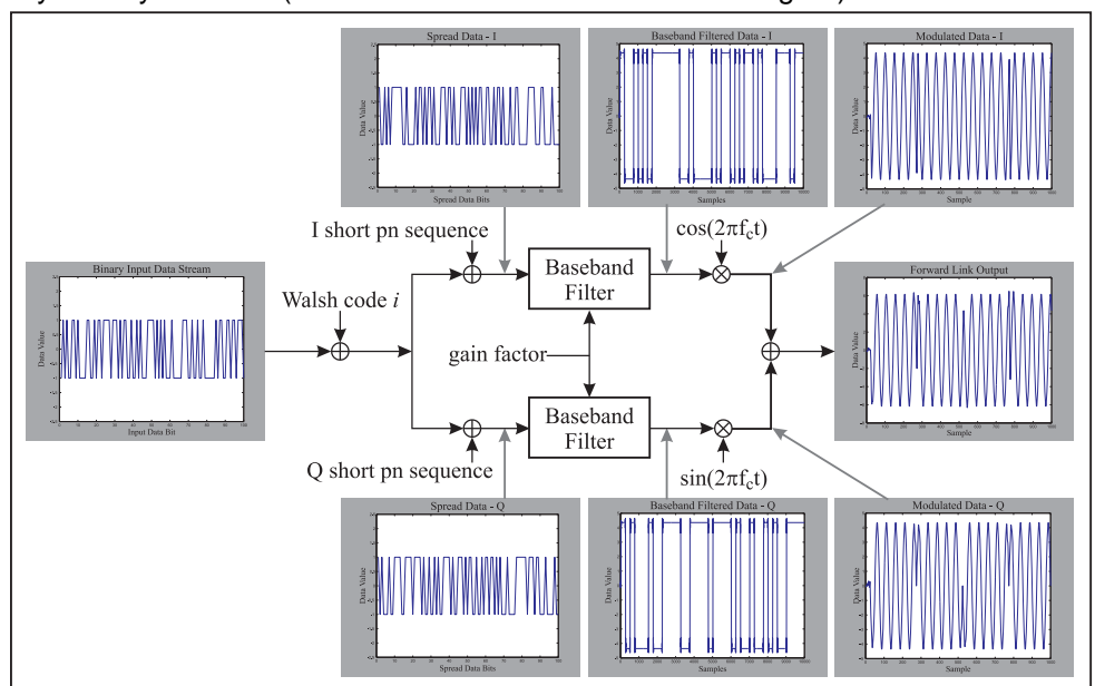
Figure 1. Simplified PCS co-channel interference model showing typical waveforms for the CDMA forward-link process.
