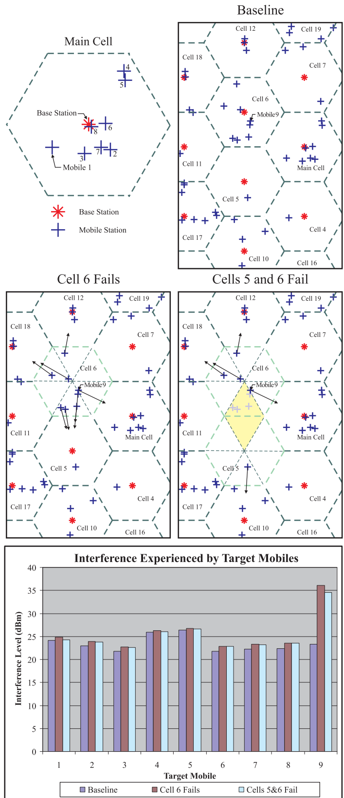
Figure 2. Typical system load analysis scenario utilizing ITS' PCS co-channel interference model.
