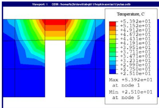
Figure 1. Temperature distribution due to heat pulse.
