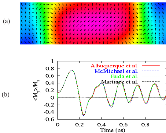
Snapshot of the magnetization during reversal (a) and (b) magnetization dynamics from Standard Problem #4.
