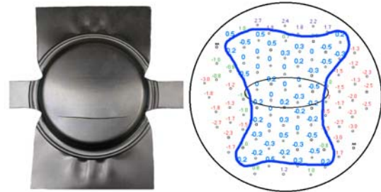
Figure 2. NIST plane-strain geometry and uniformity plot.
