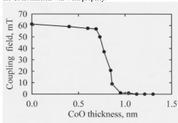
A dramatic decrease in the coupling field occurs as the pinholes disappear with increasing CoO film thickness, preventing proper operation of a GMR device.
