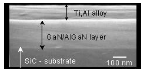
Fig 2. FE-SEM image of the (Ti:Al)/GaN cross-section
