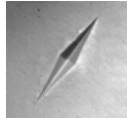
Magnified view of Knoop indentation in a new gold microhardness test block developed for the electronics industry.
