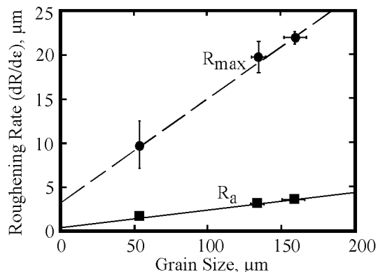
The influence of grain size on the rate of surface roughening of Al alloy 5052 deformed uniaxially.
