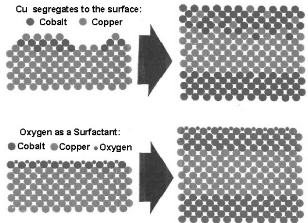
Effect of oxygen on the deposition of cobalt on copper.
