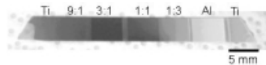
Fig 1. GaN strip with array of Ti:Al metallization pads
