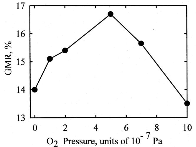
Improved performance of a GMR device results from use of a carefully selected oxygen pressure.
