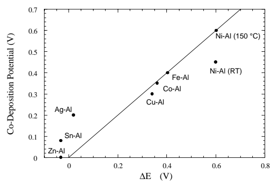
Experimentally observed co-deposition potentials versus the calculated \Delta E_{\text{Al}} values for alloys having a composition of 0.01 atomic fraction aluminum.
