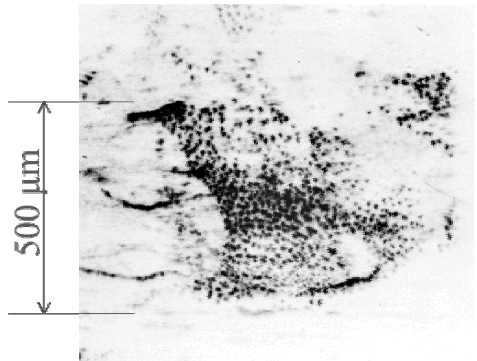
Figure 1: USAXS image of creep cavities in copper.
