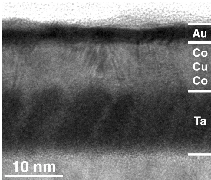
Fig. 2. Microstructure of a Co/Cu/Co spin valve deposited on 7.5 nm of Ta deposited 60° off normal. Note the corrugated interface between the Ta and the Co.
