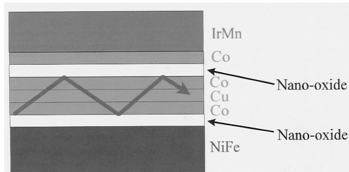
Geometry of a typical GMR material.
