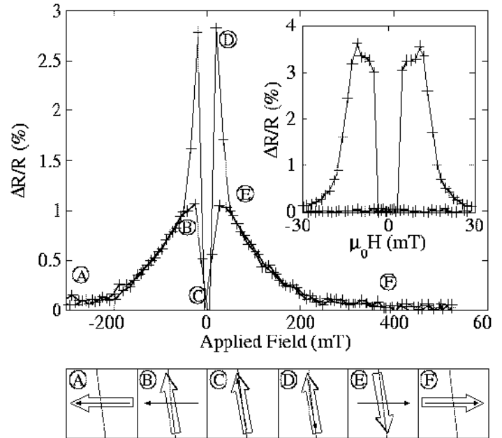
Fig. 4. Magnetoresistance of a spin valve measured with fields applied near the hard axis, and in the inset with fields applied near the easy axis. Below, a series of panels illustrating the magnetization configuration deduced from the hard axis data for the free film (thin solid arrow) and the pinned film (open arrow).
