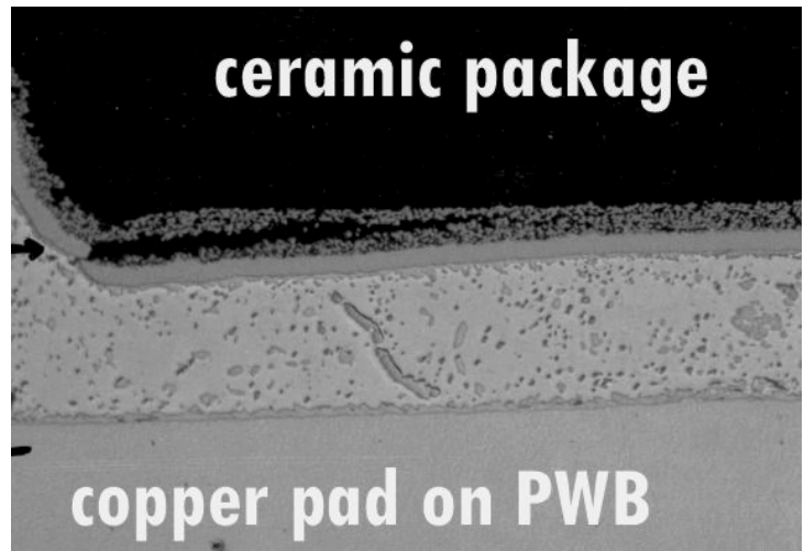
Metallographic cross-section of a new lead-free solder developed under the NCMS High-Temperature Fatigue Resistant Solder project. The alloy has excellent thermal fatigue properties.
