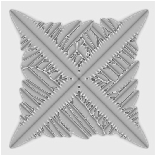
Figure 1: Two dimensional Phase field
