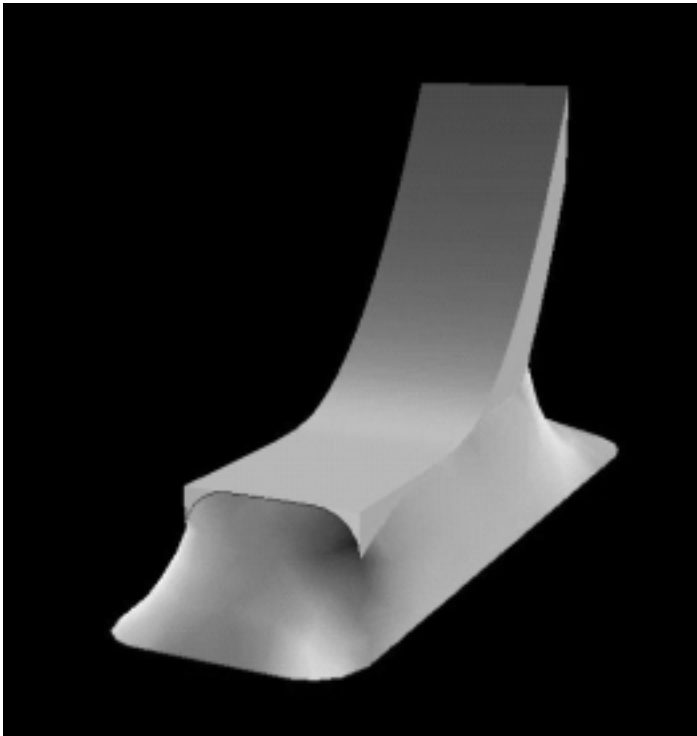
Surface Evolver calculation of the geometry of solder wetting a gull-wing lead. The shape of the liquid surface depends on the surface energy and the contact angle with the substrate.
