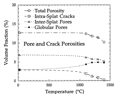
YSZ (APS Amdry 142, 90 mm spray distance) Effect of Heat Treatment (from MSANS)
