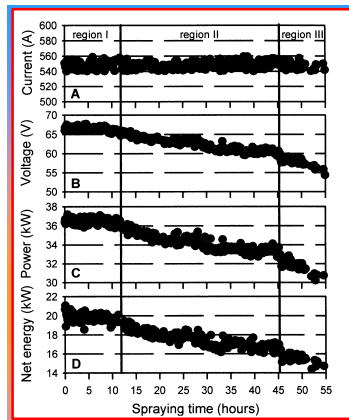
Evolution of the plasma gun parameters during 55 hours of spraying using the nominal operating conditions (constant arc current). Arc current (A) and DC voltage (B) are used in the calculation of the gun power (C) and plasma net energy (D).
