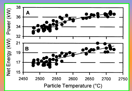
Correlation between particle temperature, gun power (A) and plasma net energy (B).
