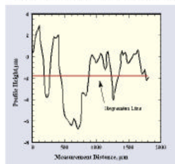
Schematic Surface Roughness Profile
