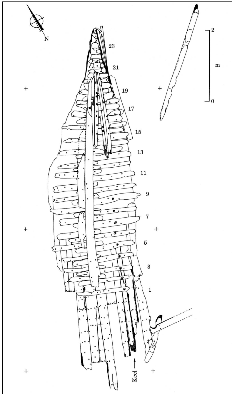
FIGURE 6. Plan of the surviving remains of the mid-fifteenth century shipwreck discovered during dredging of the Ria de Averno, Portugal (Site plan courtesy of Miguel Aleluia).
