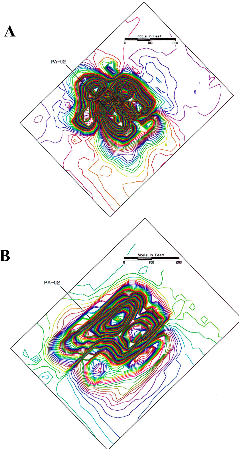
FIGURE 16. Magnetic signature of the Civil War ironclad USS Patapsco sunk in Charleston Harbor, South Carolina contoured from data recorded on 75-ft line spacing (A) and 150 ft line spacing (B) (Image courtesy of Tidewater Atlantic Research, Inc.).
