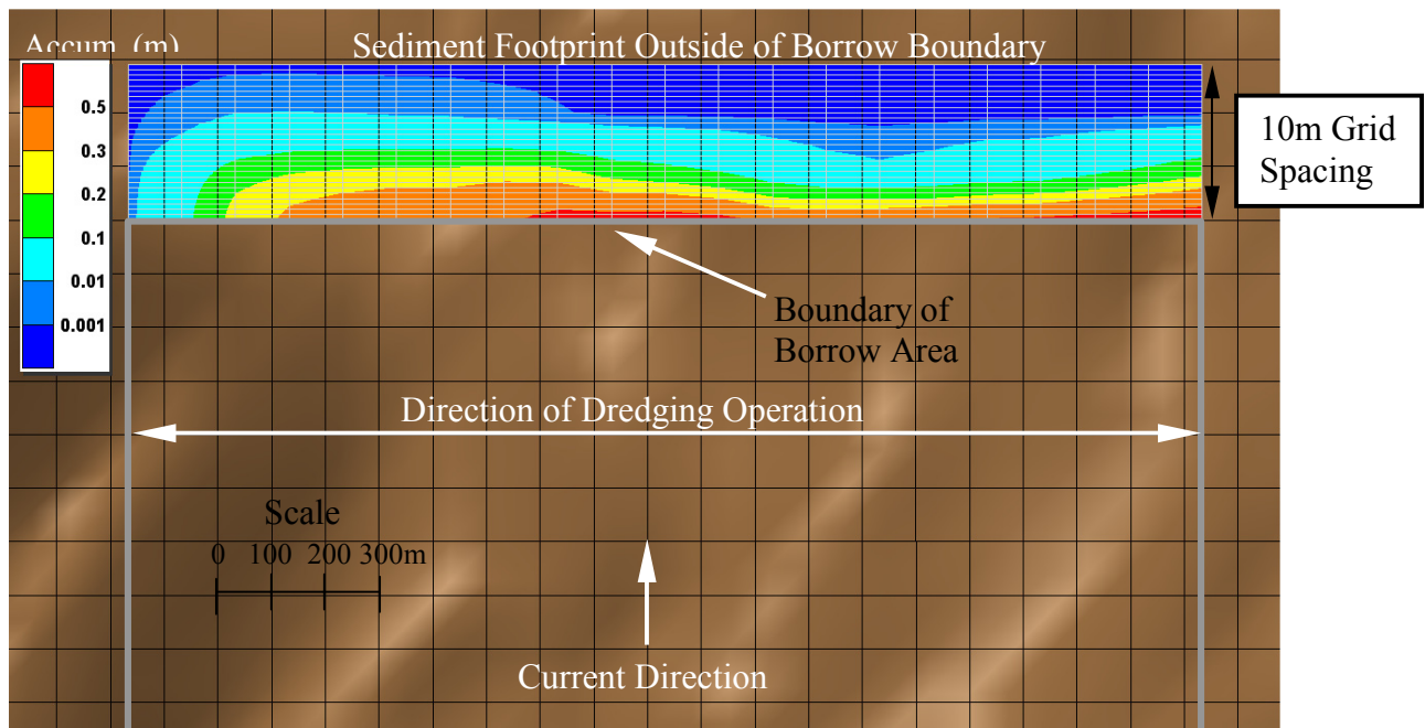
FIGURE C-1. Predicted sedimentation for a 2 million m 3 dredging operation (the larger grid squares have a 100 m dimension).
