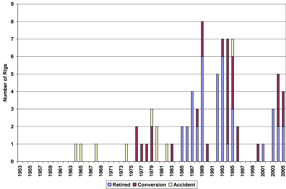
Figure D.7. Semisubmersible Attrition Rates (Kellock, 2006).
