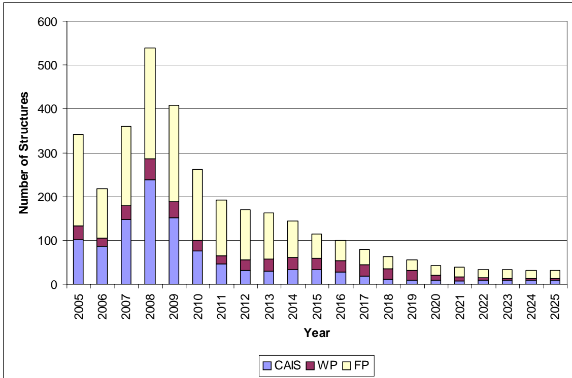
Figure B.1. Central GOM Structure Removal Model (I) Forecast.
