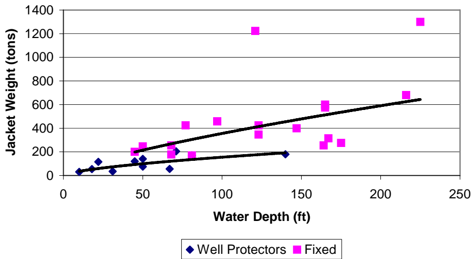
Figure E.12. Jacket Weight as a Function of Water Depth (Well Protectors and Fixed Platforms).
