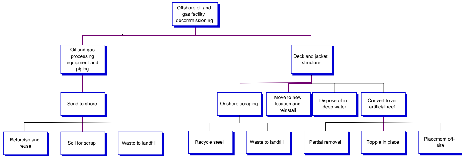
Figure C.10. Offshore Oil and Gas Facility Decommissioning Tree.
