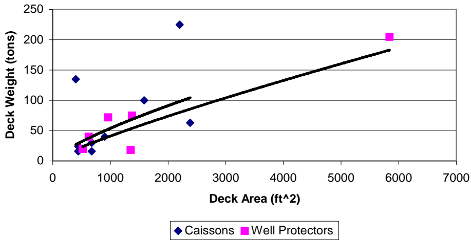
Figure E.11. Deck Weight as a Function of Deck Area (Caissons and Well Protectors).
