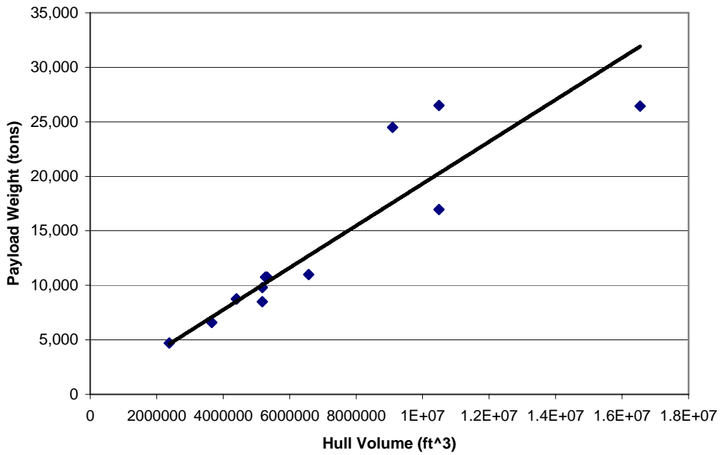
Figure E.7. Spars Payload Weight as a Function of Hull Volume.
