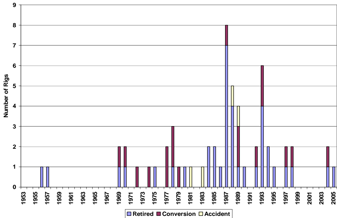
Figure D.8. Drillship Attrition Rates (Kellock, 2006).
