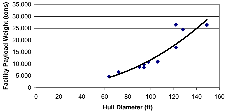
Figure E.6. Spars Facility Payload Weight as a Function of Hull Diameter.
