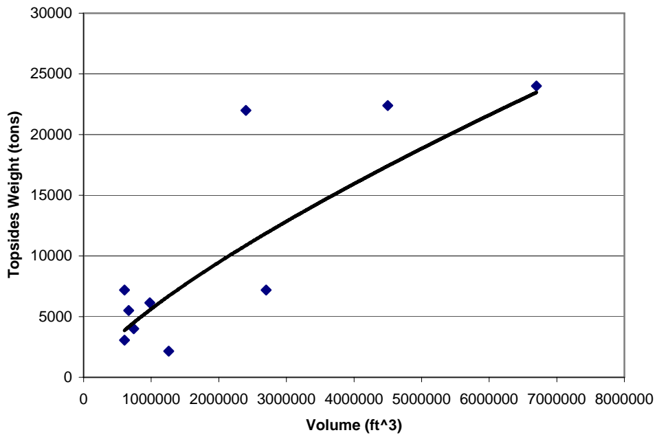
Figure E.9. TLPs Topsides Weight as a Function of Volume.
