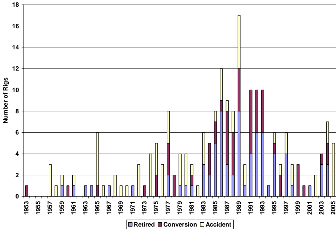
Figure D.6. Jackup Attrition Rates (Kellock, 2006).
