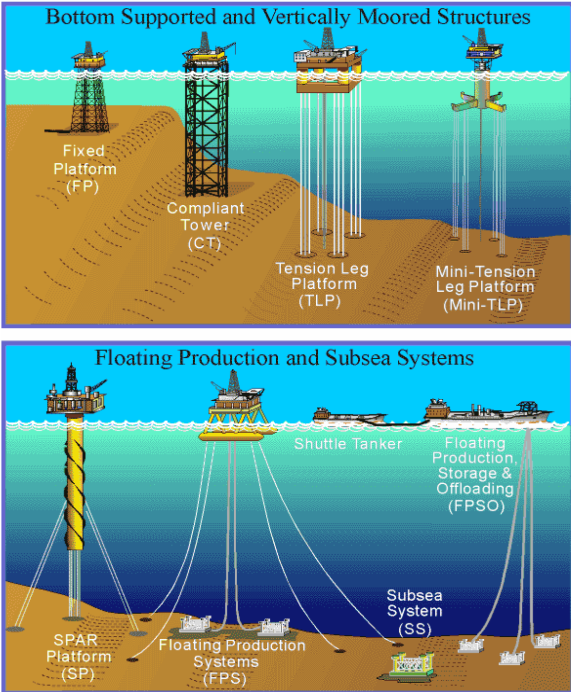
Figure A.3. Deepwater Development Strategies (French et al., 2006).
