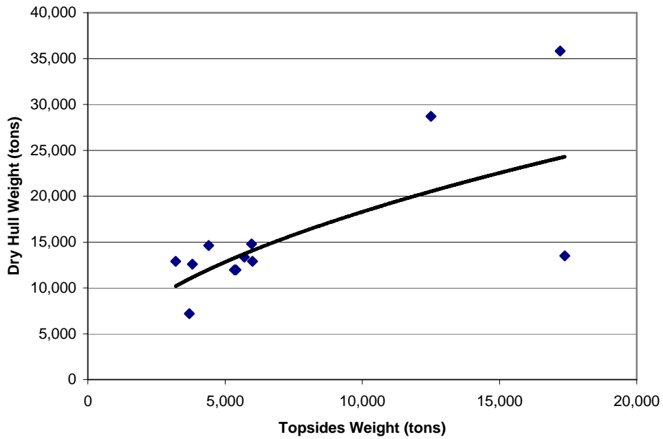
Figure E.8. Spars Dry Hull Weight as a Function of Topsides Weight.
