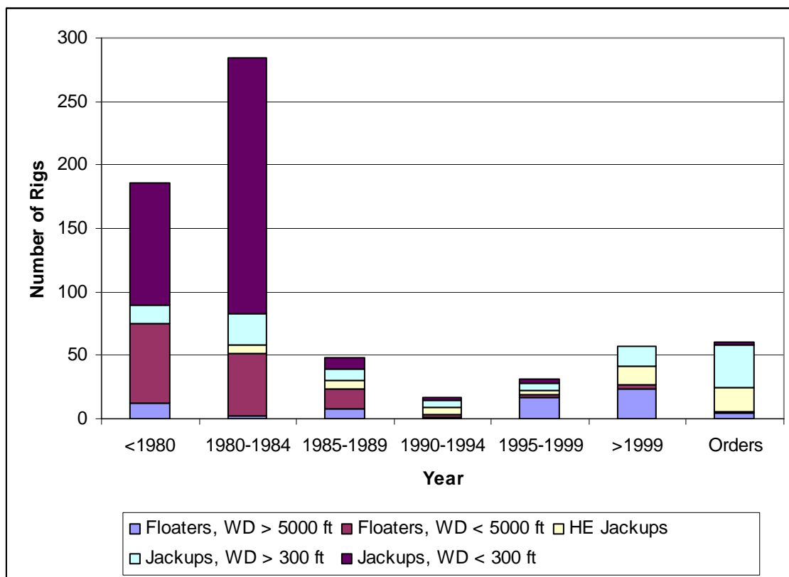
Figure D.4. Age Profile for Drilling Rig Fleet (ODS-Petrodata, 2006).
