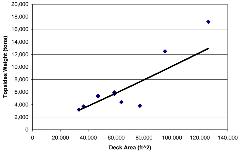
Figure E.5. Spars Topsides Weight as a Function of Deck Area.
