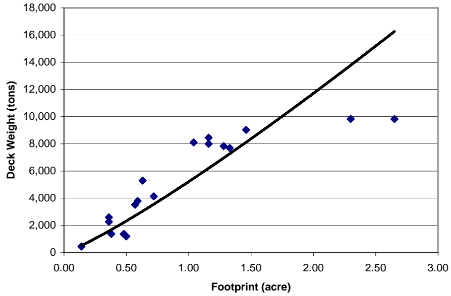
Figure E.14. Deck Weight as a Function of Jacket Footprint (Pacific Coast).
