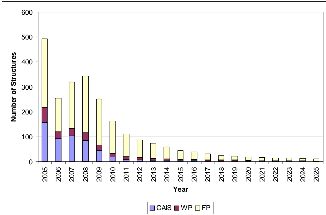
Figure B.2. Central GOM Structure Removal Model (II) Forecast.
