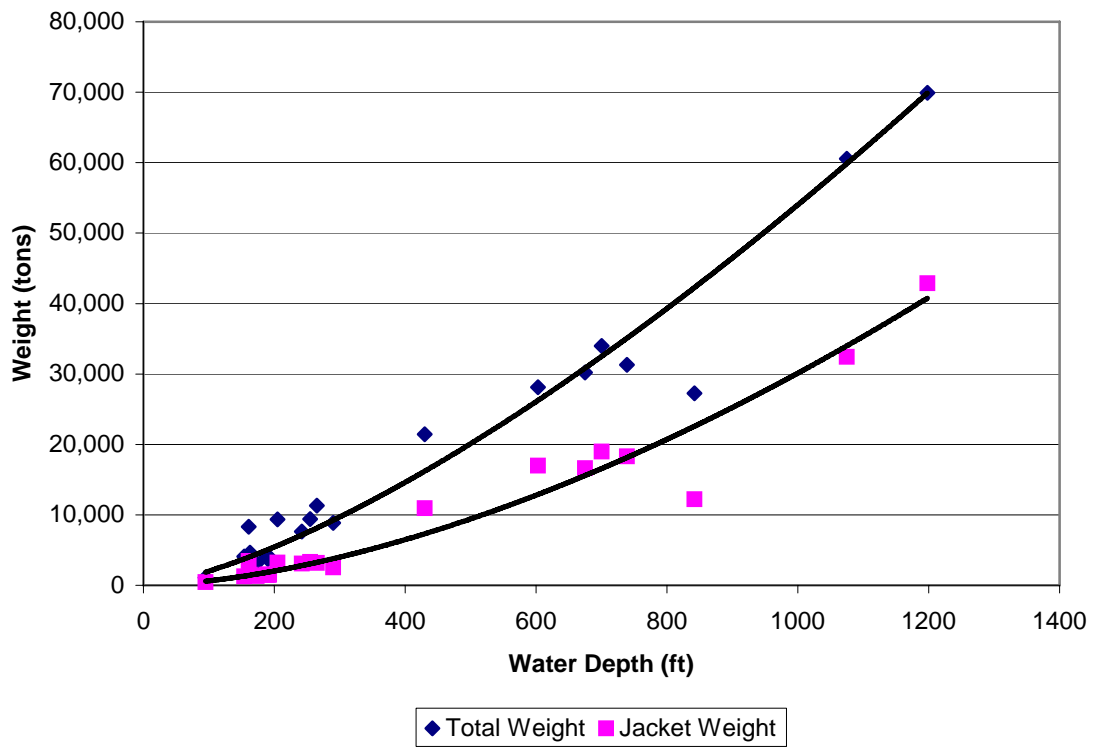
Figure E.13. Total Weight and Jacket Weight as a Function of Water Depth (Pacific Coast).
