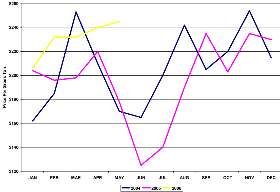
Figure C.3. Weekly No. 1 Heavy Melting Steel Scrap Price Composite (American Metal Market, 2006).
