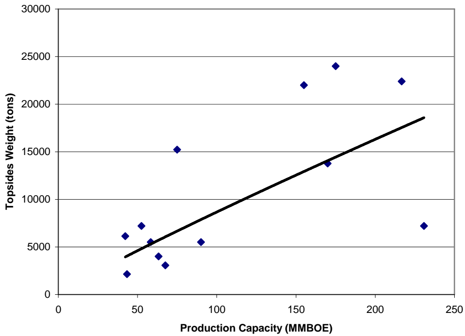
Figure E.10. TLPs Topsides Weight as a Function of Production Capacity.
