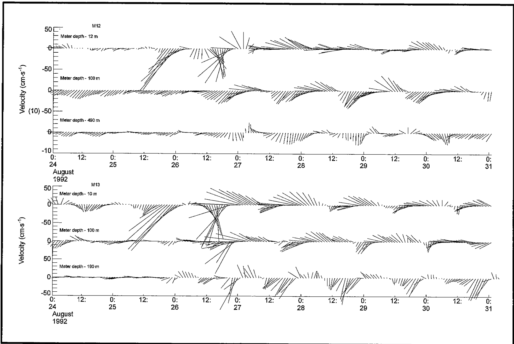
Figure 4.6. Horizontal current vectors (hourly values from 3-hr low-passed records) during late August 1992 from two locations off Louisiana at approximately 90.5^{\circ}\text{W} on the shelf edge and upper slope. The cross-shelf components are oriented up and down (up is on shore) and along shelf components are oriented across the figure (generally eastward to the right). Moorings 13 and 12 were located in water depths of 200 and 504 m; current meter depths are indicated. The eye of Hurricane Andrew passed on a northeastward track approximately 85 km north of mooring 13 at about 0000 UTC on 26 August.
