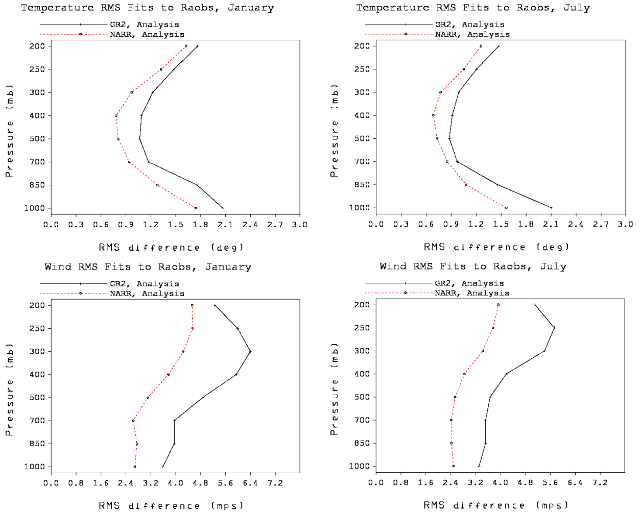
Fig. 6. Rms fits to rawinsondes as a function of pressure, for temperature (upper panels), and for vector wind (lower panels), for January (left panels) and July (right panels), averages over 1979-2002. NARR: dashed lines, GR2: solid lines.
