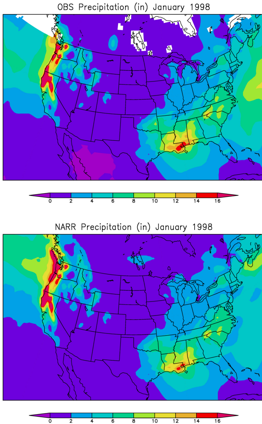
Fig 3. "Observed" (analyzed) precipitation assimilated by the NARR over land and over low and lower mid-latitude oceans (see text), and NARR precipitation, averaged for January 1998 (inches/month). White indicates no available observations.
