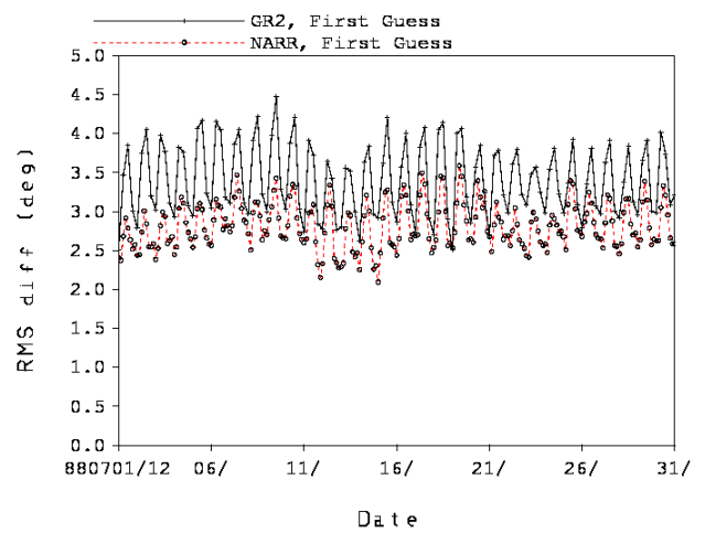
2-m Temp. RMS Fits to SFC Data, July 1988
