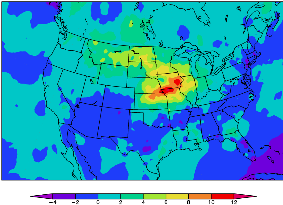
Fig. 4. Difference between 1993 and 1988 of the monthly average precipitation over June-July (inches/month) for the "observed" precipitation, assimilated by the NARR over land and over low and lower mid-latitude oceans (see text), and the NARR precipitation.
