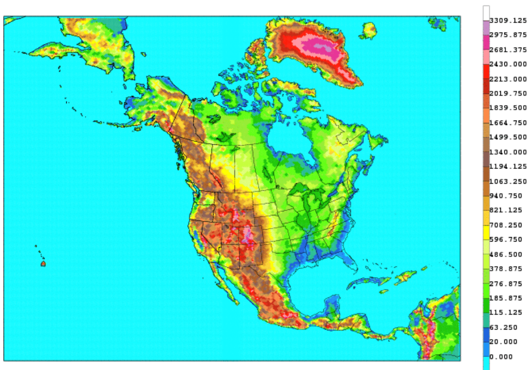
Fig. 2. The NCEP Regional Reanalysis domain and its 32 km topography. Terrain elevation (m) is indicated by the color scale at the right.
