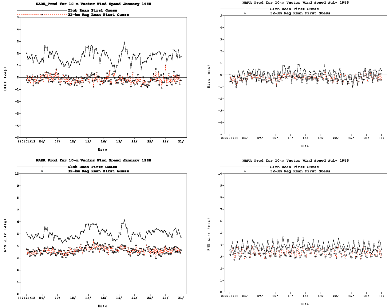
Fig. 7. Same as Fig. 6 but for the 10-m winds
