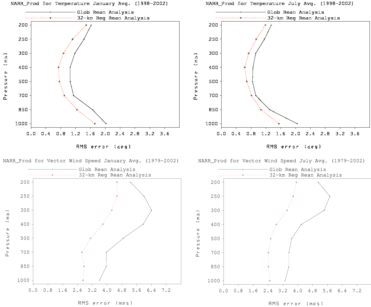
Fig. 4. RMS fits to rawinsondes as a function of pressure, for temperature (upper panels), and for vector wind (lower panels), for January (left panels) and July (right panels), average over 1998-2002 for temperature, and over 1979-2002 for wind. NARR: dashed lines, GR: solid lines.
