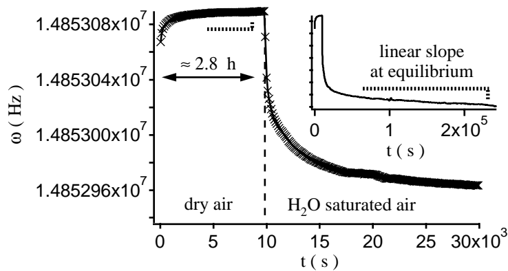
Figure 4. Typical QCM frequency shift data is shown for 3 rd overtone of the resonant frequency in both dry and moisture saturated air. The inset, whose vertical axis is the same as the main part of the figure, extends the data to very long times to demonstrate the linear drift in the signal at equilibrium. The accuracy to which \omega is determined is better than 0.1 Hz.
