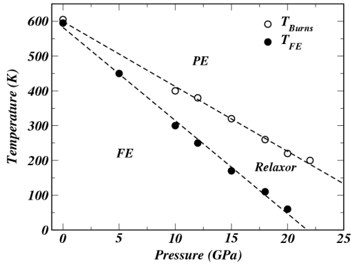
FIG. 5: Predicted pressure vs. temperature phase diagram for PSN, indicating the ferroelectric to relaxor transition, and the estimated Burns temperature.
