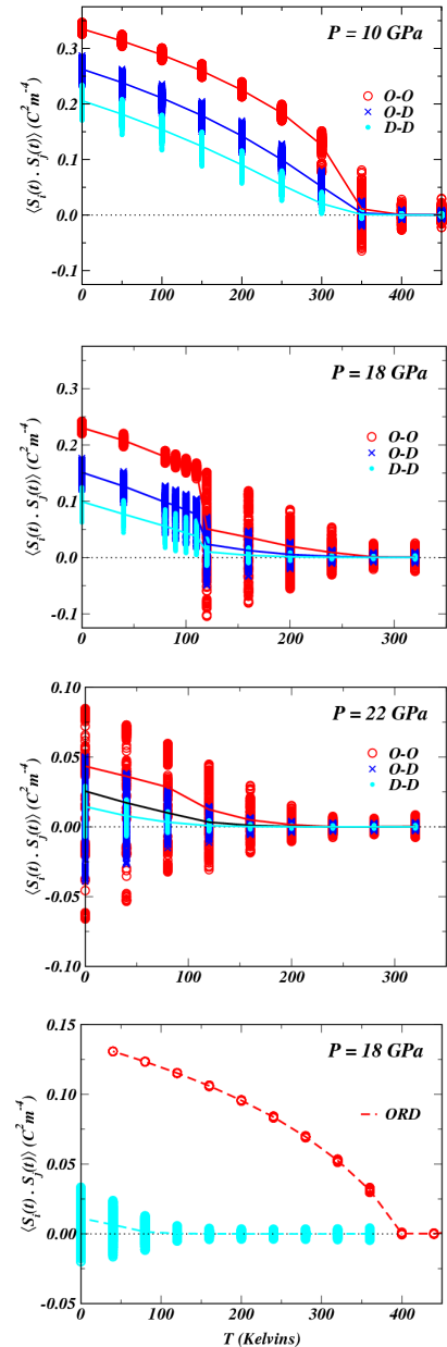
FIG. 4: (Color online) PSN cluster-polarization dot products as functions of temperature: O-O indicate products between moments of two chemically ordered clusters, \langle \vec{S}_O(t) \cdot \vec{S}_{O'}(t) \rangle ; O-D for products between one chemically ordered- and one disordered cluster, \langle \vec{S}_O(t) \cdot \vec{S}_D(t) \rangle ; D-D is for two disordered clusters, \langle \vec{S}_D(t) \cdot \vec{S}_{D'}(t) \rangle . Lines link average products. (a) at 10 GPa the relaxor region is small. (b) at 18 GPa there is a substantial relaxor region above a first-order phase transition. (c) at 22 GPa the transition is suppressed, and only the relaxor region persists. (d) Is a plot of the P=18 GPa results for: an ideally ordered system (above) which has no quenched local fields; and a chemically random configuration (below).
