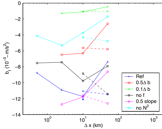
Fig. 15. The final buoyancy of the overflow b_f , following mixing and entrainment, shown as a function of resolution for each of the six different cases. z -coordinate calculations are shown with solid lines, isopycnal coordinate calculations are shown with dashed lines. The asterisk shows the result for the 10 km horizontal resolution isopycnal calculation with increased vertical viscosity.
