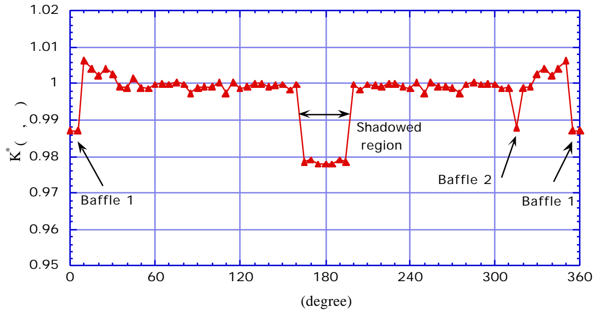
Figure 4. The SRDF ( \theta = 90^\circ ) of the NIST 2.5 m integrating sphere obtained by the computer simulation.
