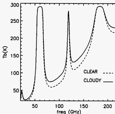
Figure 1. Calculated brightness temperatures (K) from 20 to 220 GHz for clear and cloudy conditions. The clear calculations are based on a standard atmosphere with the surface values ( S ) of P_S = 1013 mb, T_S = 293 K, \rho_S = 10 \text{ gm}^{-3} , and IWV = 2.34 cm. The cloudy atmosphere contains 1 mm of integrated cloud liquid with a cloud layer of liquid density of 0.1 \text{ gm}^{-3} between 1 and 2 km. The absorption models used are given in Figure 2.
