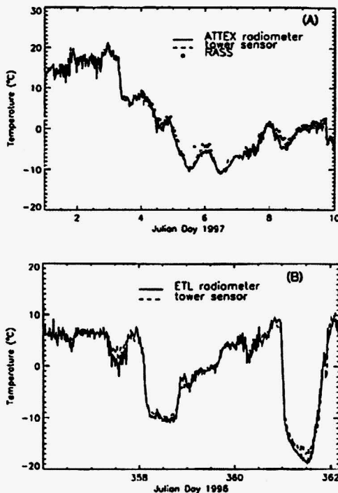
Figure 10. (A) A 10-day time series of temperature at 200 m as measured by the ATTEX radiometer, by the in situ measurement on the tower, and by a Radio Acoustic Sounding System (RASS). January 1–10, 1997. (B) A 6-day time series of temperature at 200 m as measured by the ETL radiometer and by the in situ measurement on the tower. December 21–27, 1996. After [40].
