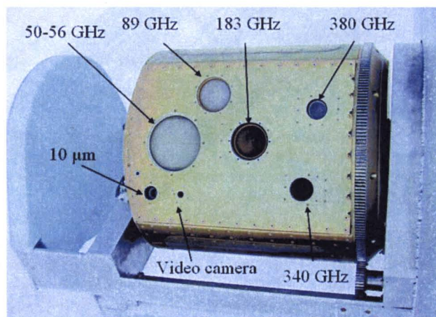
Figure 5. Photograph of the scanhead of the GSR.
