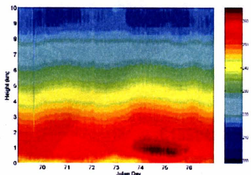
Figure 9. Time-height cross-sections derived from MWRP data during the NSA/AAO Arctic Winter Radiometric Experiment that was conducted in Barrow, Alaska, USA, during March-April 2004.
