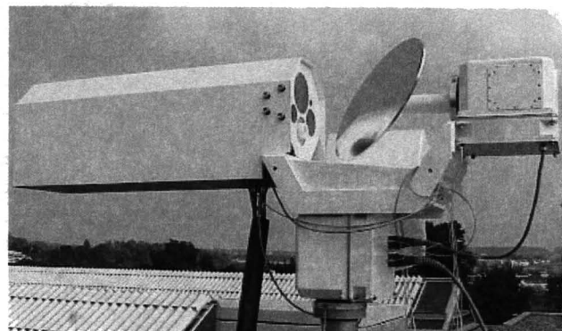
Figure 3. ASMUWARA in operation the IAP in Bern, Switzerland. The openings of the 4 horns appear as grey disks at the left of the rotatable mirror, while the IR radiometer looks through the white cylinder below the largest horn.
