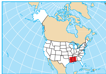
Albers equal area projection
