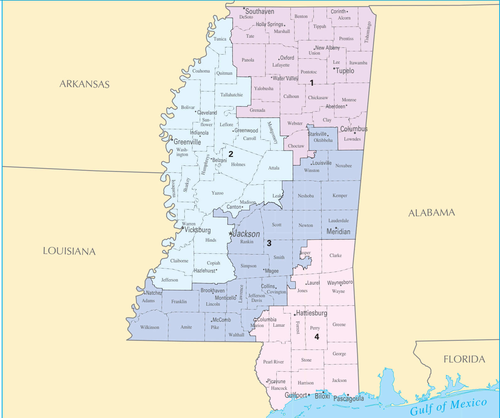
Albers equal area projection
