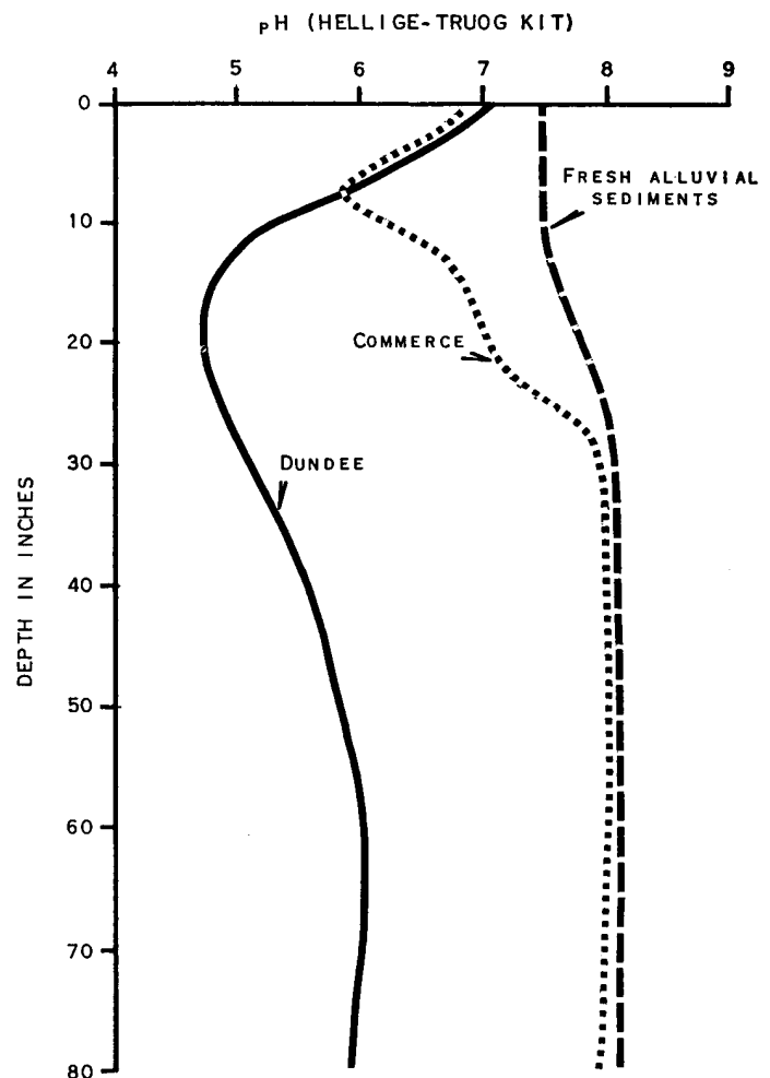
Figure 8.—pH of soils of differing ages.
