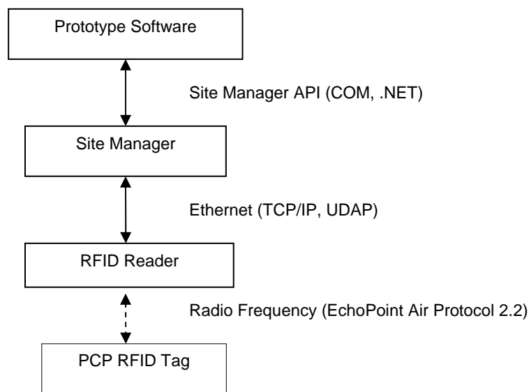
Figure 7. The software structure for the RFID system
