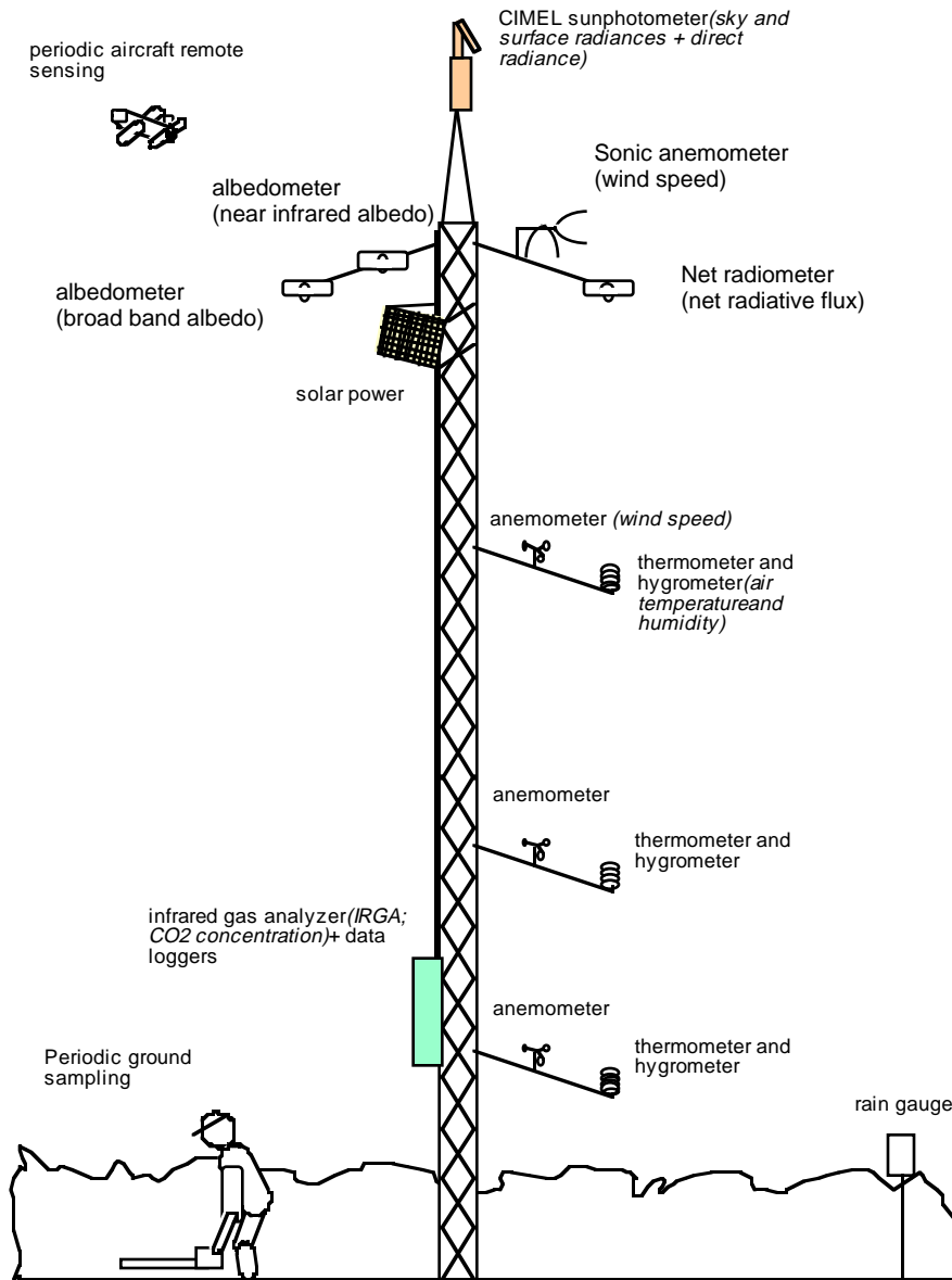
Figure 2: Tower schematic
