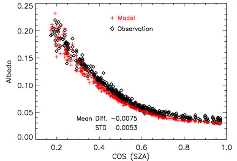
Model and Observation Comparison For Ocean Surface Albedo at COVE (3-1-00 to 3-1-01)
