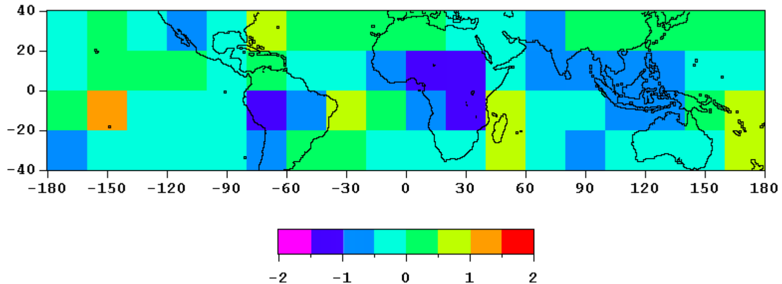
ADM monthly mean flux biases ( \text{W m}^{-2} ) over 20^\circ \times 20^\circ regions from CERES/TRMM SSF Edition 2 SW TOA fluxes.
