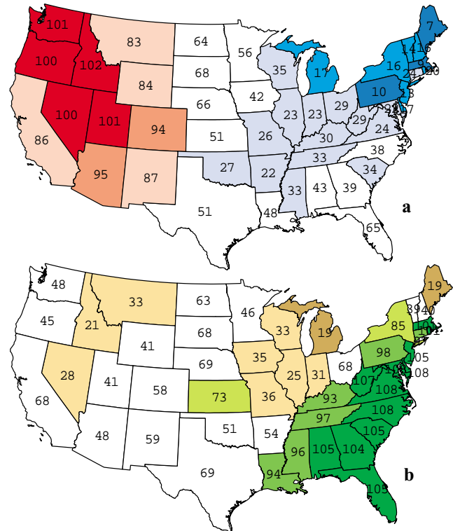
Fig. 1. October 2002 - June 2003: statewide ranks of (a) temperature and (b) precipitation. A rank of 1 represents the coldest or wettest period, and a rank of 108 indicates the warmest or driest period, in the 108-yr record between 1895-2003.
