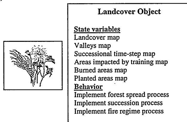
Figure 3. Landcover Object State Variables and Behaviors
