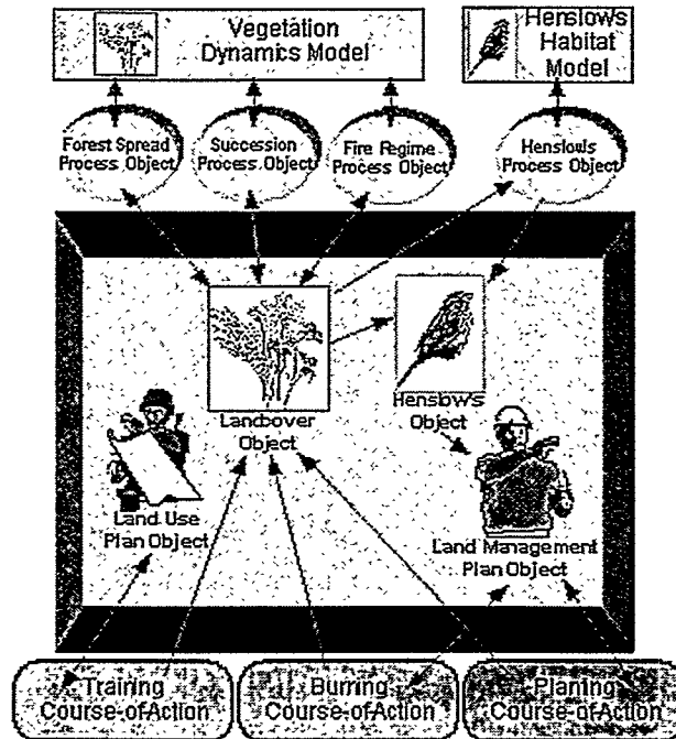
Figure 2. OO-IDLAMS Prototype Conceptual Design
