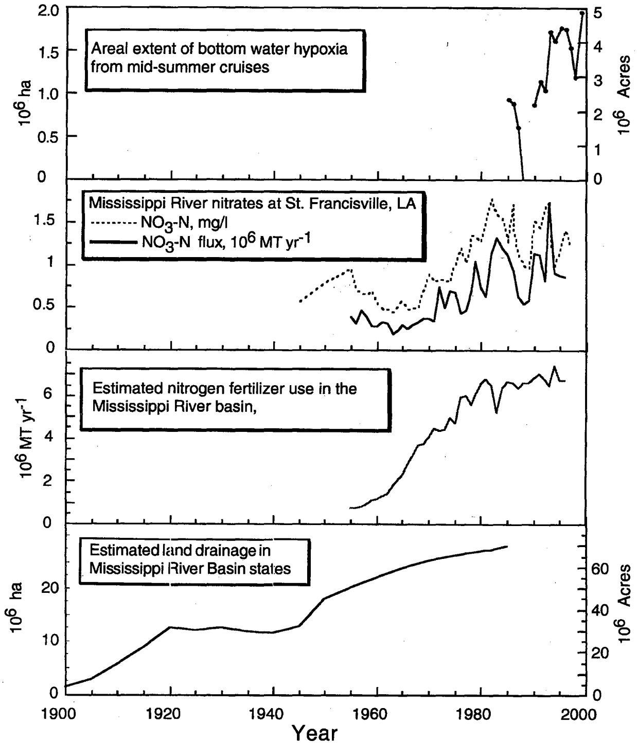
FIGURE I.2. Estimated trends in the 20th century of the hypoxia area, nitrogen concentrations and fluxes, nitrogen fertilizer use, and land drainage in the Mississippi River Basin. (Data from Rabalais et al. 1999, Goolsby et al. 1999, and USDA 1987.)
