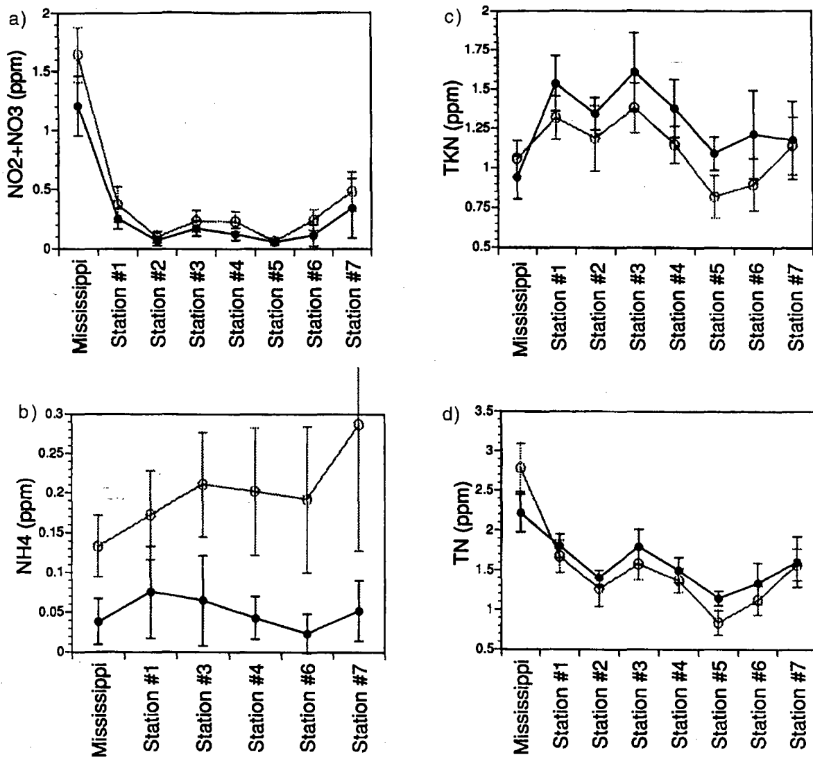
FIGURE 3.24. Pre- and post-diversion data with standard error bars for Louisiana's Breton Sound Estuary for (a) nitrite + nitrate, (b) ammonium-nitrogen, (c) total Kjeldahl nitrogen, and (d) total nitrogen. NOTE: Solid black data points are pre-diversion; open data points are post-diversion.
