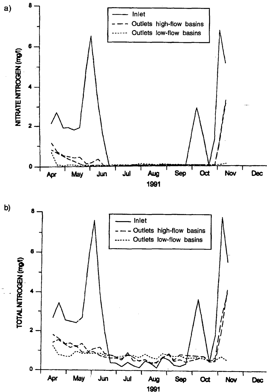
FIGURE 3.7. A strong seasonal pattern of nitrate–nitrogen and total nitrogen typical of mid-western U.S. streams was seen with high concentrations in the spring and fall (inlet data) from the Des Plaines River. NOTE: Outflows are from one low-flow (EW 4) and two high-flow (EW 3 and 5) wetland basins at the Des Plaines Wetland Demonstration Project, shown in Figure 3.6. (From Phipps and Crumpton 1994.)
