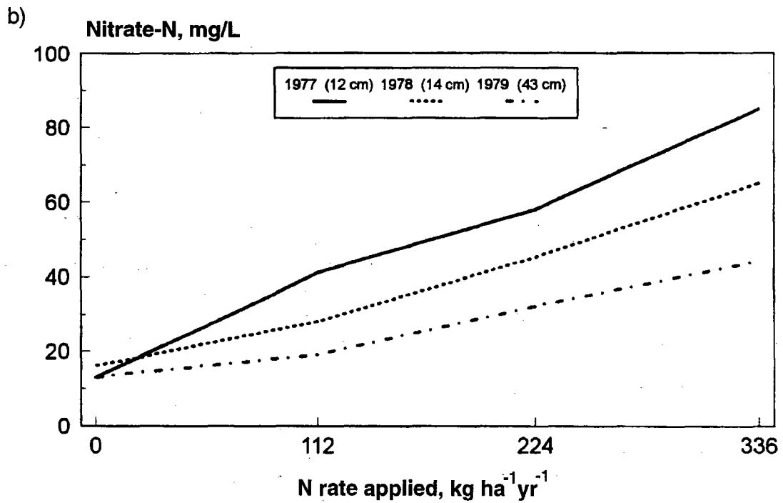
FIGURE 3.2. Nitrate-nitrogen concentration in tile-drainage water as affected by rate of N-fertilizer application for continuous corn at (a) Lamberton and (b) Waseca, MN.
