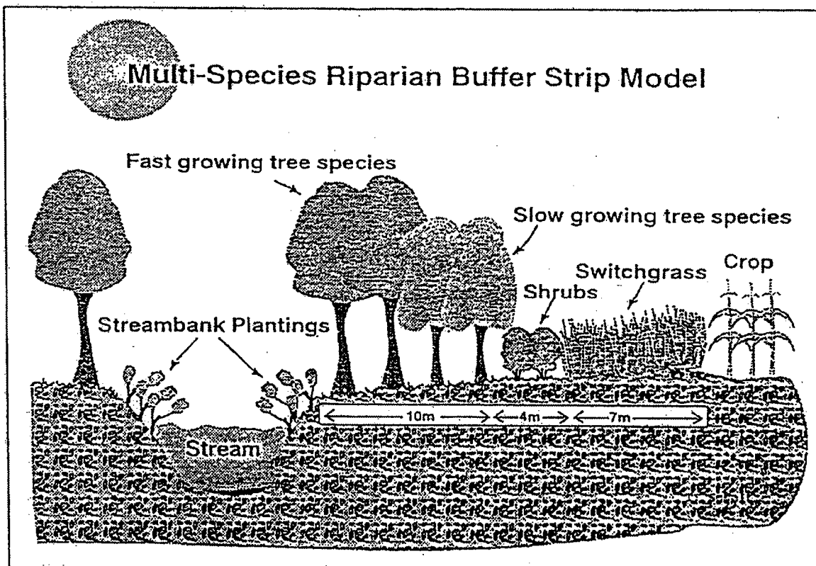
FIGURE 3.15. Schematics of riparian buffer zones: (a) three-zone riparian buffer system (from Welsch 1991), and (b) multi-species riparian buffer strip model which includes tree rows closest to the stream, shrubs, and a strip of switchgrass adjacent to the cropland. (From R. Schultz.)
