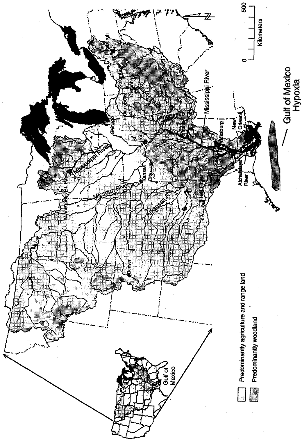
FIGURE I.1. The Mississippi River Basin and location of the Gulf of Mexico hypoxia. (Adapted from Goolsby et al. 1999.)
