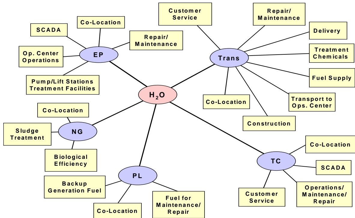
Figure 2: Water and wastewater interdependencies
