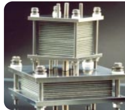
MSRI's solid oxide fuel cell stack
