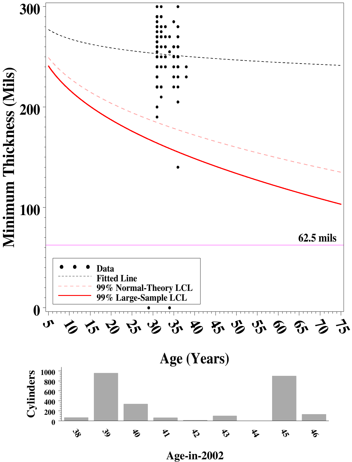
Figure 16. Minimum thicknesses and cylinder age distribution for ETTP, Thin, top and bottom, pre-FY98.
