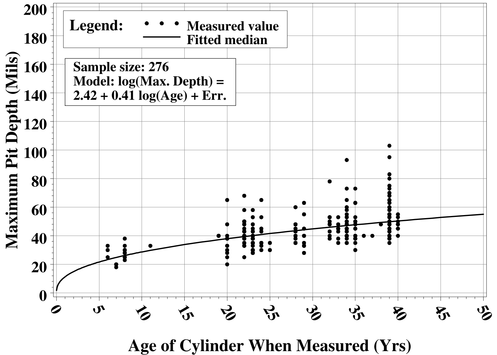
Figure 6. Pit depth estimates for PORTS, top, pre-FY98.
