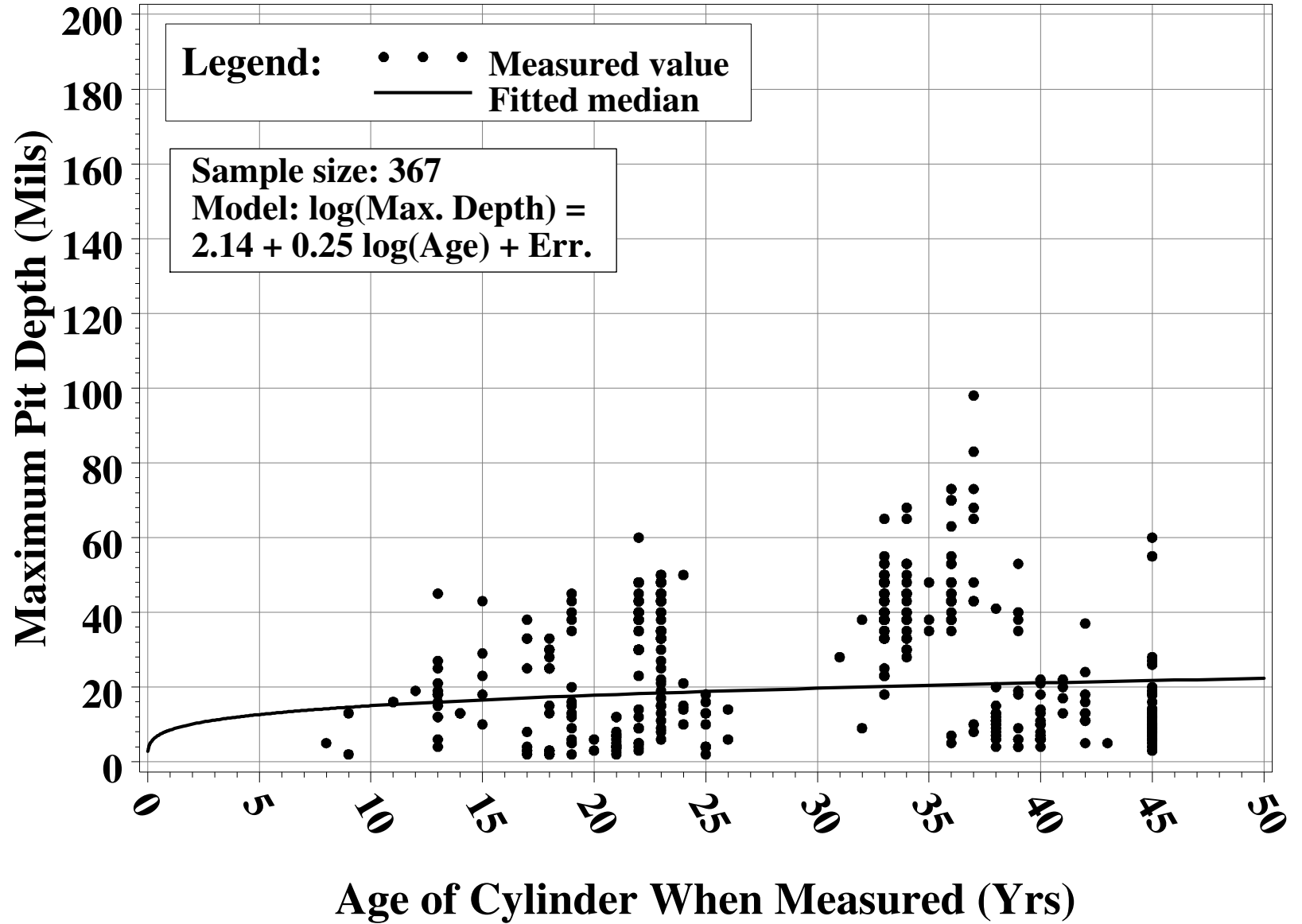
Figure 5. Pit depth estimates for PGDP top.
