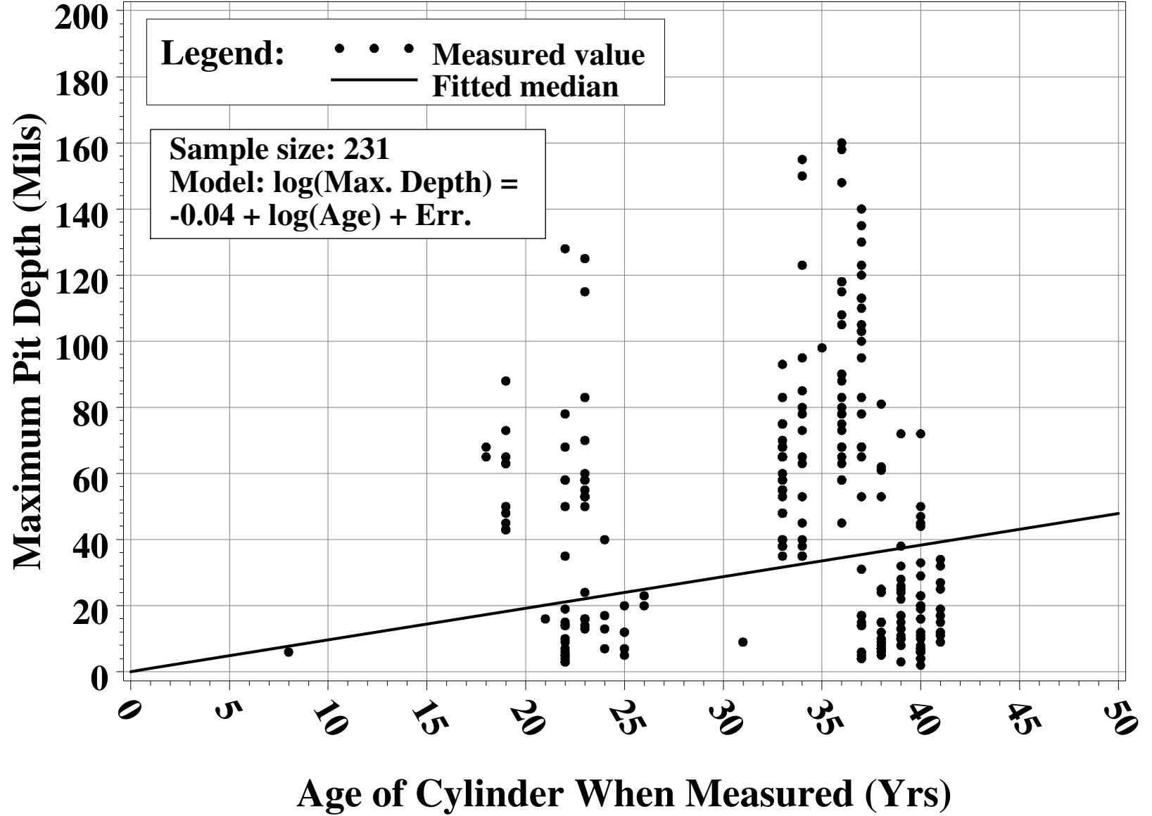
Figure 3. Pit depth estimates for C-745-G, bottom.
