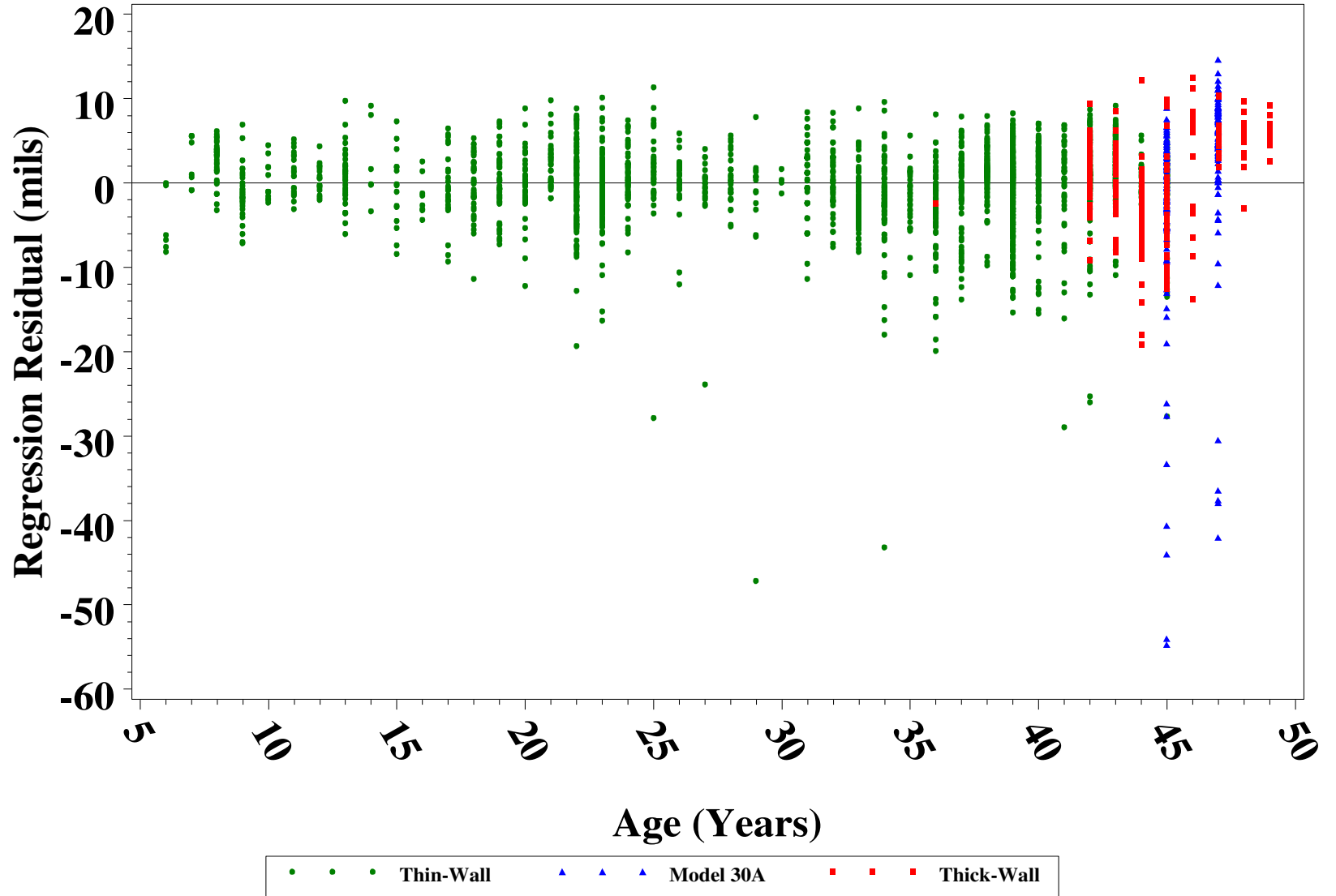
Figure 31. Residuals from minimum thickness regression.
