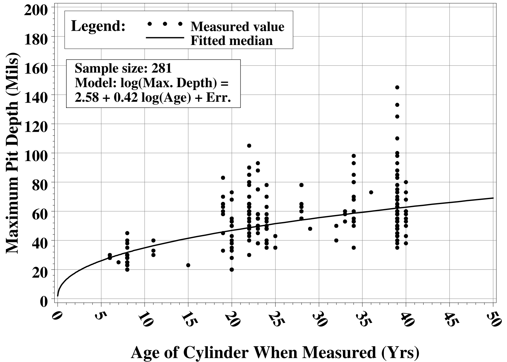
Figure 7. Pit depth estimates for PORTS bottom, pre-FY98.
