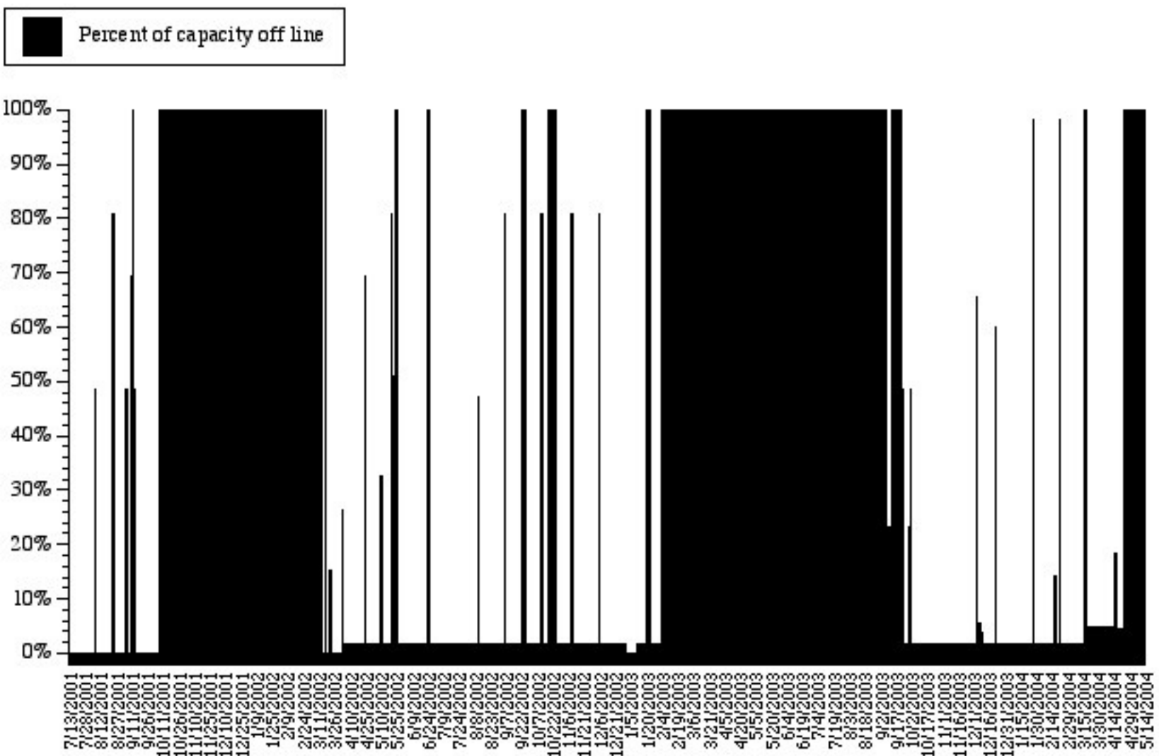
Figure 1. Hunters Point Power Plant Unit 4 Outage Profile, July 13, 2001 through May 14, 2004
